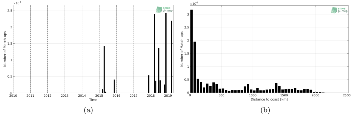
Figure 1: Number of match-ups between TSG-SAMOS and SMAP-L3-RSS-V4-8DAY-RUNNING SSS as a function of time (a) and as function of the distance to coast (b) over the Tropical Atlantic Ocean Pi-MEP region and for the full satellite product period.
