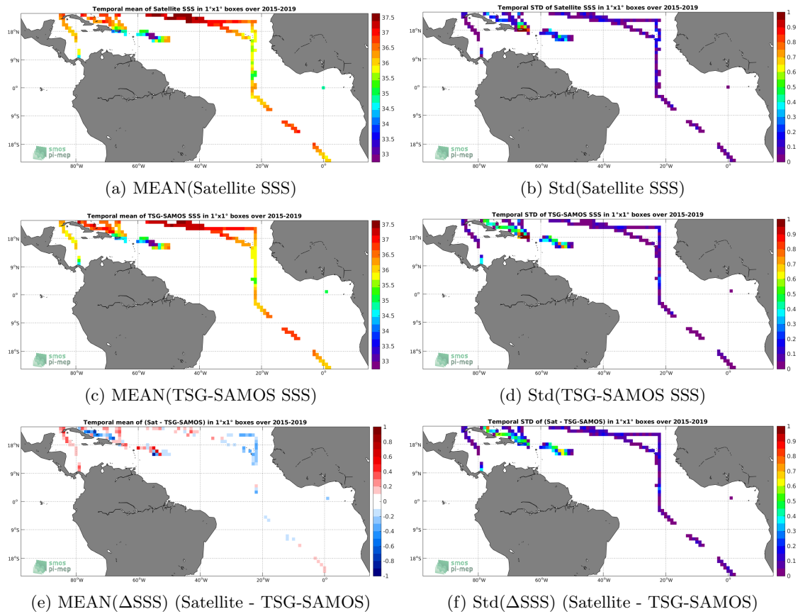
Figure 6: Temporal mean (left) and Std (right) of SSS from SMAP-L3-RSS-V4-8DAY-RUNNING (top), TSG-SAMOS (middle), and of \Delta SSS (Satellite - TSG-SAMOS). Only match-up pairs are used to generate these maps.
