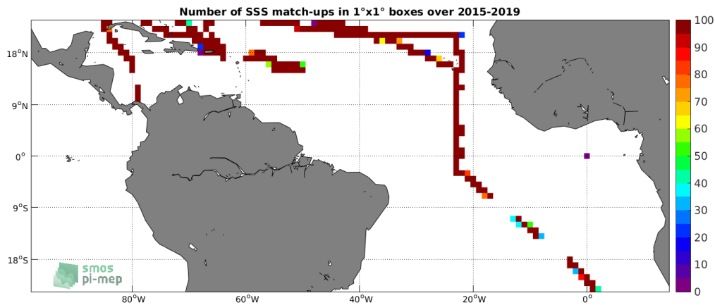
Figure 4: Number of SSS match-ups between TSG-SAMOS SSS and the SMAP-L3-RSS-V4-8DAY-RUNNING SSS product for the Tropical Atlantic Ocean Pi-MEP region over 1^\circ \times 1^\circ boxes and for the full satellite product period.
