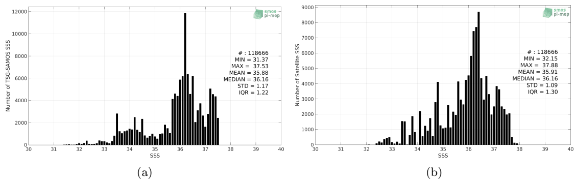
Figure 2: Histograms of SSS from TSG-SAMOS (a) and SMAP-L3-RSS-V4-8DAY-RUNNING (b) considering all match-up pairs per bins of 0.1 over the Tropical Atlantic Ocean Pi-MEP region and for the full satellite product period.
