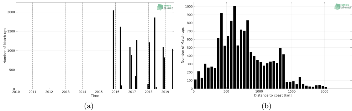
Figure 1: Number of match-ups between TSG (Polarstern) and SMAP SSS L3 v4 - 8-Day running (RSS) SSS as a function of time (a) and as function of the distance to coast (b) over the Tropical Atlantic Ocean Pi-MEP region and for the full satellite product period.
