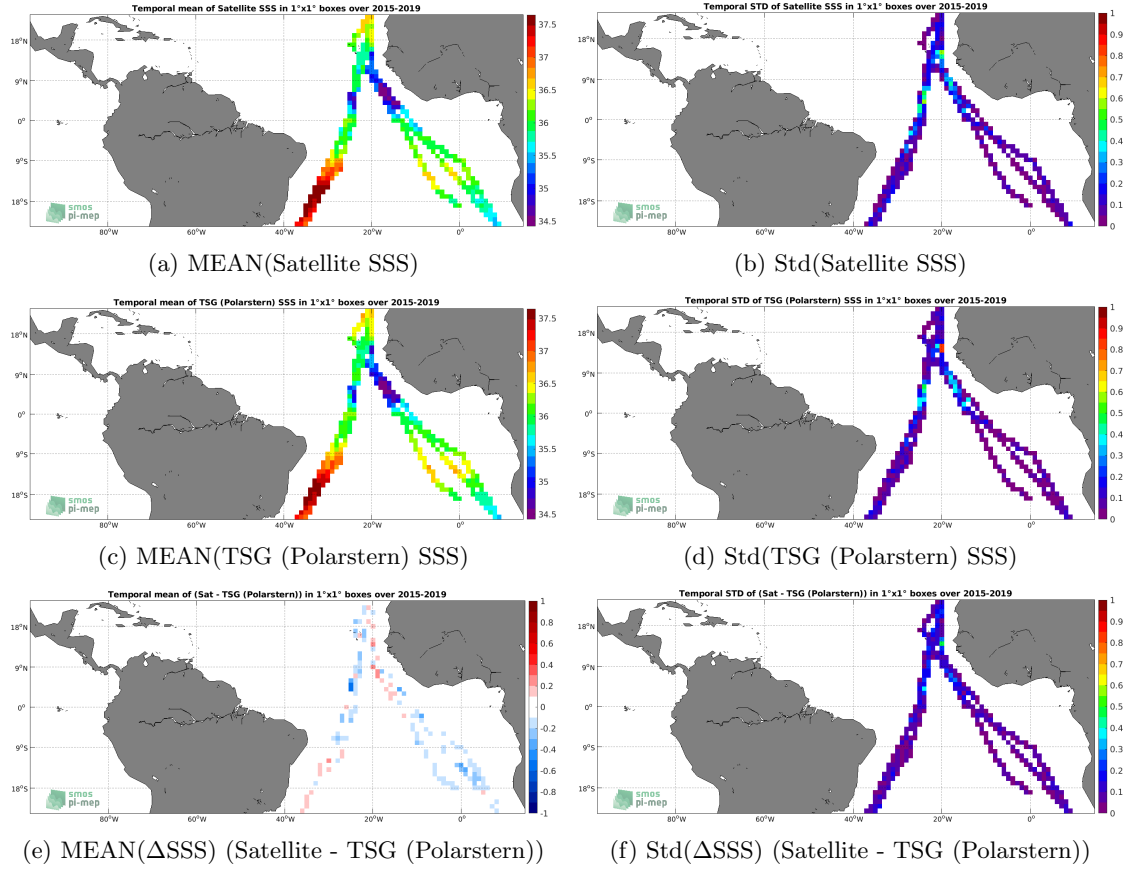
Figure 6: Temporal mean (left) and Std (right) of SSS from SMAP SSS L3 v4 - 8-Day running (RSS) (top), TSG (Polarstern) (middle), and of \Delta SSS (Satellite - TSG (Polarstern)). Only match-up pairs are used to generate these maps.
