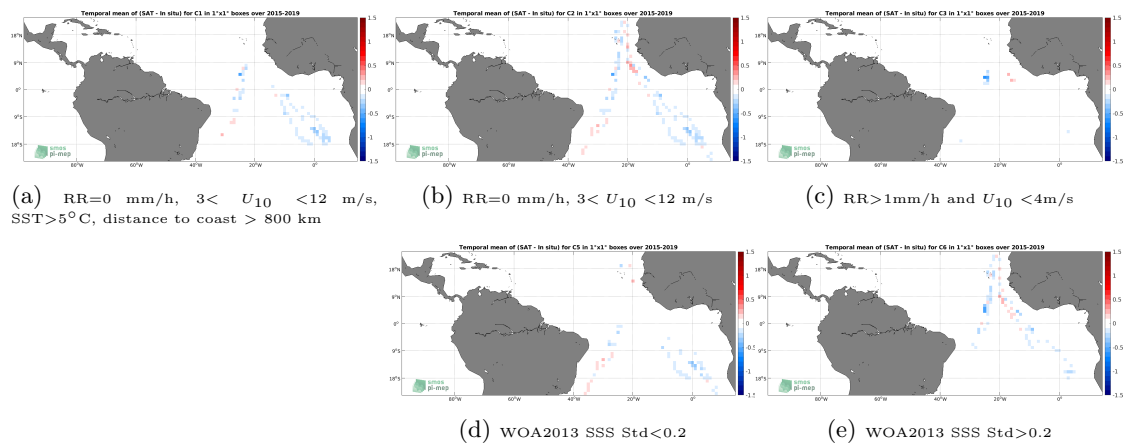
Figure 12: Temporal mean gridded over spatial boxes of size 1^\circ \times 1^\circ of \Delta SSS (SMAP SSS L3 v4 - 8-Day running (RSS) - TSG (Polarstern)) for 5 different subdatasets corresponding to:RR=0 mm/h, 3 < U_{10} < 12 m/s, SST > 5^\circ\text{C} , distance to coast > 800 km (a), RR=0 mm/h, 3 < U_{10} < 12 m/s (b), RR > 1 mm/h and U_{10} < 4 m/s (c), WOA2013 SSS Std < 0.2 (d), WOA2013 SSS Std > 0.2 (e).
