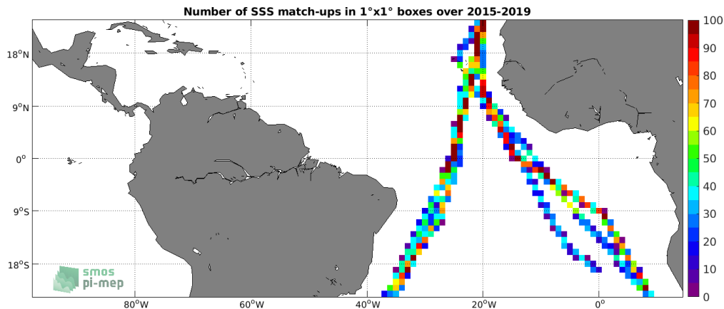
Figure 4: Number of SSS match-ups between TSG (Polarstern) SSS and the SMAP SSS L3 v4 - 8-Day running (RSS) SSS product for the Tropical Atlantic Ocean Pi-MEP region over 1^\circ \times 1^\circ boxes and for the full satellite product period.
