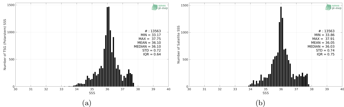
Figure 2: Histograms of SSS from TSG (Polarstern) (a) and SMAP SSS L3 v4 - 8-Day running (RSS) (b) considering all match-up pairs per bins of 0.1 over the Tropical Atlantic Ocean Pi-MEP region and for the full satellite product period.
