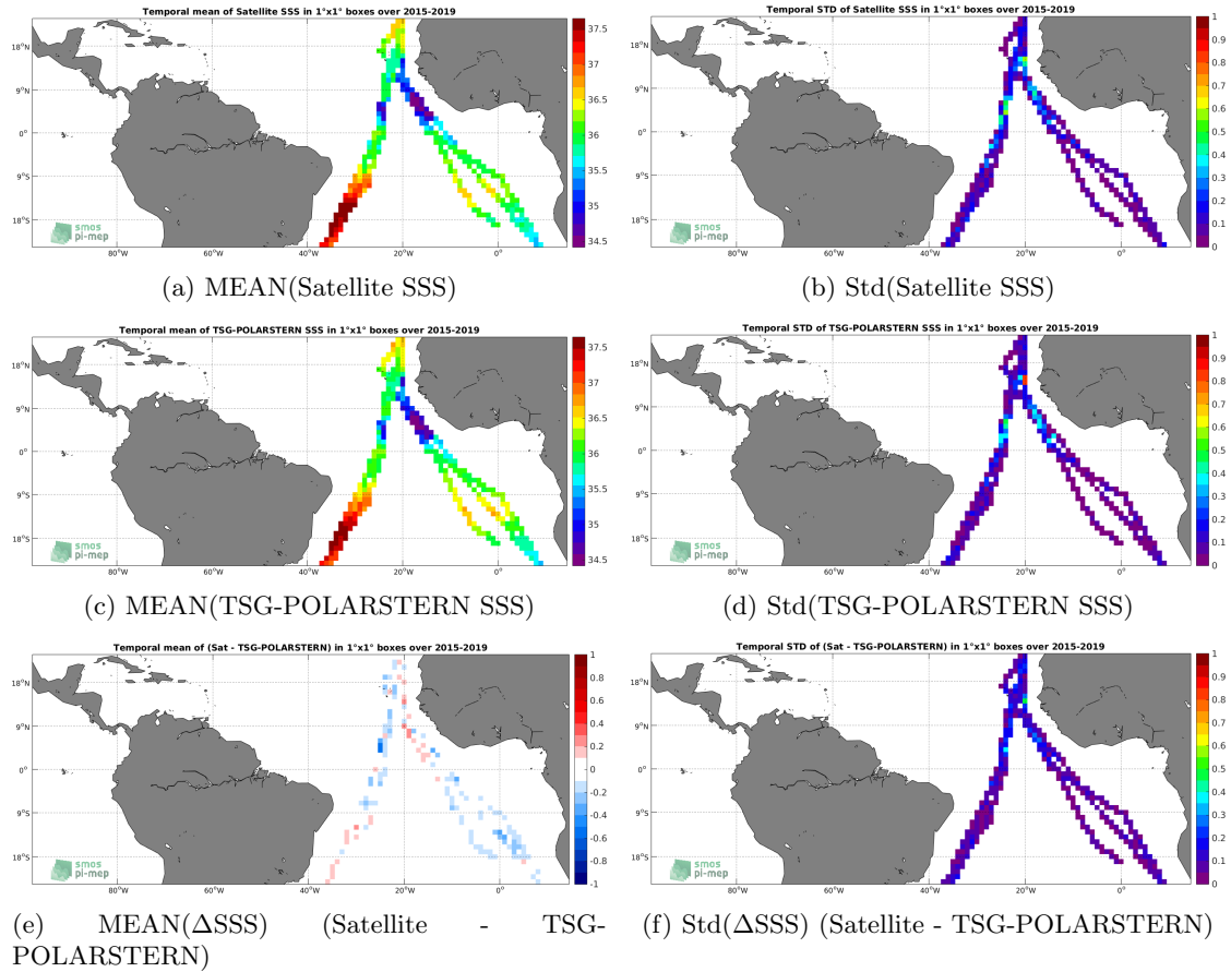
Figure 6: Temporal mean (left) and Std (right) of SSS from SMAP-L3-RSS-V4-8DAY-RUNNING (top), TSG-POLARSTERN (middle), and of \Delta SSS (Satellite - TSG-POLARSTERN). Only match-up pairs are used to generate these maps.
