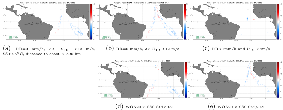
Figure 12: Temporal mean gridded over spatial boxes of size 1^\circ \times 1^\circ of \Delta SSS (SMAP-L3-RSS-V4-8DAY-RUNNING - TSG-POLARSTERN) for 5 different subdatasets corresponding to:RR=0 mm/h, 3 < U_{10} < 12 m/s, SST >5^\circ\text{C} , distance to coast > 800 km (a), RR=0 mm/h, 3 < U_{10} < 12 m/s (b), RR >1 mm/h and U_{10} < 4 m/s (c), WOA2013 SSS Std <0.2 (d), WOA2013 SSS Std >0.2 (e).
