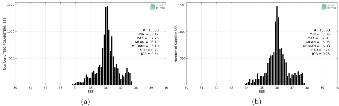
Figure 2: Histograms of SSS from TSG-POLARSTERN (a) and SMAP-L3-RSS-V4-8DAY-RUNNING (b) considering all match-up pairs per bins of 0.1 over the Tropical Atlantic Ocean Pi-MEP region and for the full satellite product period.
