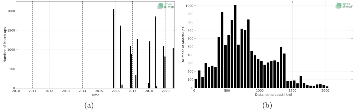
Figure 1: Number of match-ups between TSG-POLARSTERN and SMAP-L3-RSS-V4-8DAY-RUNNING SSS as a function of time (a) and as function of the distance to coast (b) over the Tropical Atlantic Ocean Pi-MEP region and for the full satellite product period.
