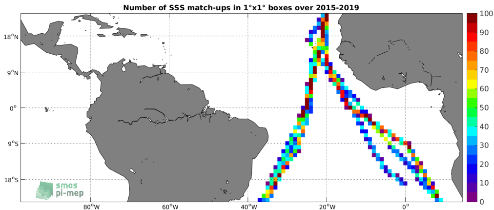
Figure 4: Number of SSS match-ups between TSG-POLARSTERN SSS and the SMAP-L3-RSS-V4-8DAY-RUNNING SSS product for the Tropical Atlantic Ocean Pi-MEP region over 1°x1° boxes and for the full satellite product period.
