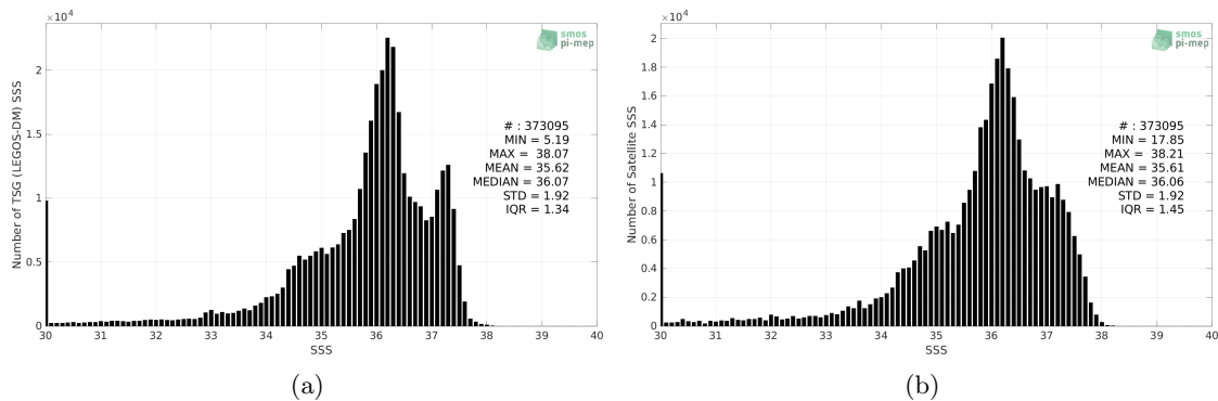
Figure 2: Histograms of SSS from TSG (LEGOS-DM) (a) and SMAP SSS L3 v4 - 8-Day running (RSS) (b) considering all match-up pairs per bins of 0.1 over the Tropical Atlantic Ocean Pi-MEP region and for the full satellite product period.
