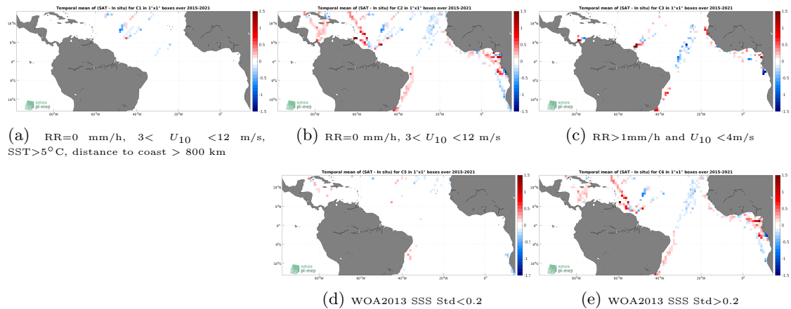
Figure 12: Temporal mean gridded over spatial boxes of size 1^\circ \times 1^\circ of \Delta SSS (SMAP SSS L3 v4 - 8-Day running (RSS) - TSG (LEGOS-DM)) for 5 different subdatasets corresponding to:RR=0 mm/h, 3 < U_{10} < 12 m/s, SST >5^\circ\text{C} , distance to coast > 800 km (a), RR=0 mm/h, 3 < U_{10} < 12 m/s (b), RR >1 mm/h and U_{10} < 4 m/s (c), WOA2013 SSS Std <0.2 (d), WOA2013 SSS Std >0.2 (e).
