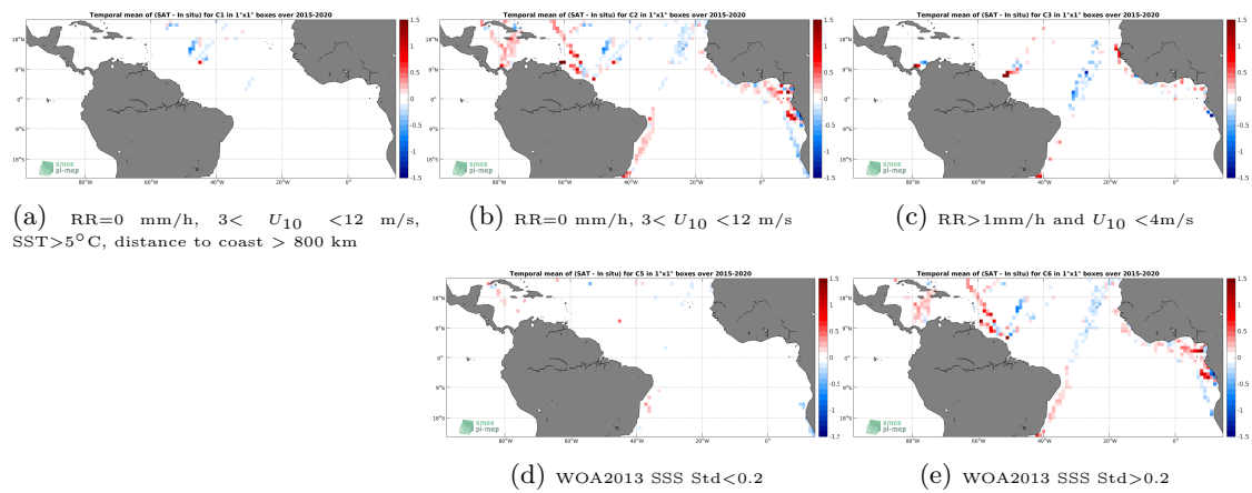
Figure 12: Temporal mean gridded over spatial boxes of size 1^\circ \times 1^\circ of \Delta SSS (SMAP SSS L3 v4 - 8-Day running (RSS) - TSG (LEGOS-DM)) for 5 different subdatasets corresponding to: RR=0 mm/h, 3 < U_{10} < 12 m/s, SST > 5°C, distance to coast > 800 km (a), RR=0 mm/h, 3 < U_{10} < 12 m/s (b), RR > 1mm/h and U_{10} < 4 m/s (c), WOA2013 SSS Std < 0.2 (d), WOA2013 SSS Std > 0.2 (e).
