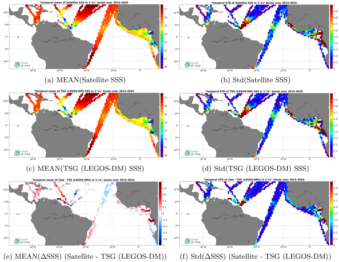
Figure 6: Temporal mean (left) and Std (right) of SSS from SMAP SSS L3 v4 - 8-Day running (RSS) (top), TSG (LEGOS-DM) (middle), and of \Delta SSS (Satellite - TSG (LEGOS-DM)). Only match-up pairs are used to generate these maps.
