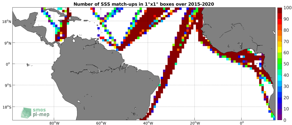
Figure 4: Number of SSS match-ups between TSG (LEGOS-DM) SSS and the SMAP SSS L3 v4 - 8-Day running (RSS) SSS product for the Tropical Atlantic Ocean Pi-MEP region over 1^\circ \times 1^\circ boxes and for the full satellite product period.
