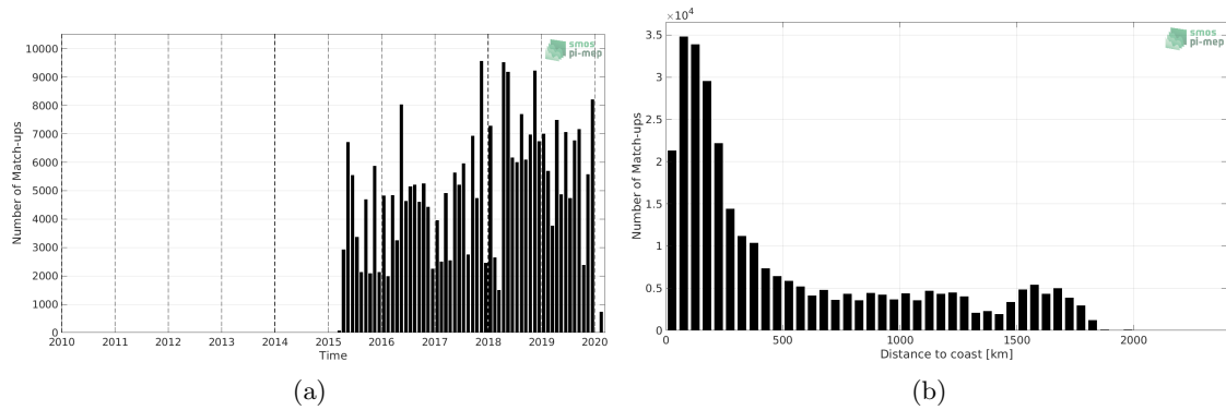
Figure 1: Number of match-ups between TSG (LEGOS-DM) and SMAP SSS L3 v4 - 8-Day running (RSS) SSS as a function of time (a) and as function of the distance to coast (b) over the Tropical Atlantic Ocean Pi-MEP region and for the full satellite product period.
