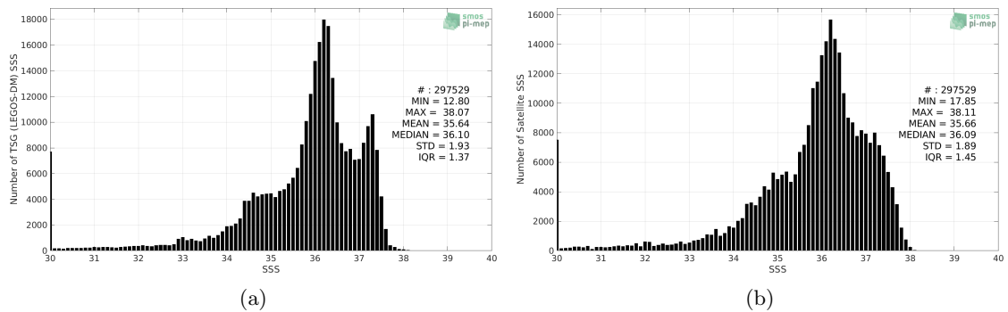
Figure 2: Histograms of SSS from TSG (LEGOS-DM) (a) and SMAP SSS L3 v4 - 8-Day running (RSS) (b) considering all match-up pairs per bins of 0.1 over the Tropical Atlantic Ocean Pi-MEP region and for the full satellite product period.
