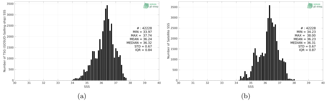
Figure 2: Histograms of SSS from TSG (GOSUD-Sailing-ship) (a) and SMAP SSS L3 v4 - 8-Day running (RSS) (b) considering all match-up pairs per bins of 0.1 over the Tropical Atlantic Ocean Pi-MEP region and for the full satellite product period.
