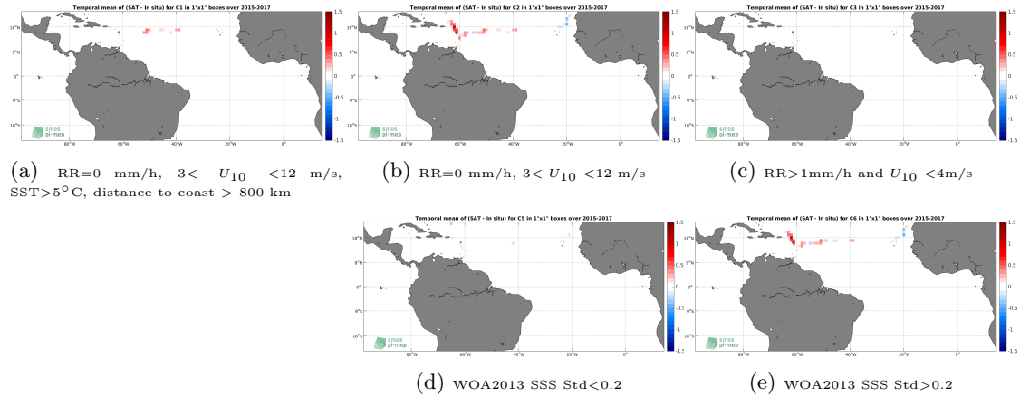
Figure 12: Temporal mean gridded over spatial boxes of size 1^{\circ}\times 1^{\circ} of \Delta SSS (SMAP-L3-RSS-V4-8DAY-RUNNING - TSG-GOSUD-Sailing-ship) for 5 different subdatasets corresponding to:RR=0 mm/h, 3 < U_{10} < 12 m/s, SST >5^{\circ}\text{C} , distance to coast > 800 km (a), RR=0 mm/h, 3 < U_{10} < 12 m/s (b), RR >1 mm/h and U_{10} < 4 m/s (c), WOA2013 SSS Std <0.2 (d), WOA2013 SSS Std >0.2 (e).
