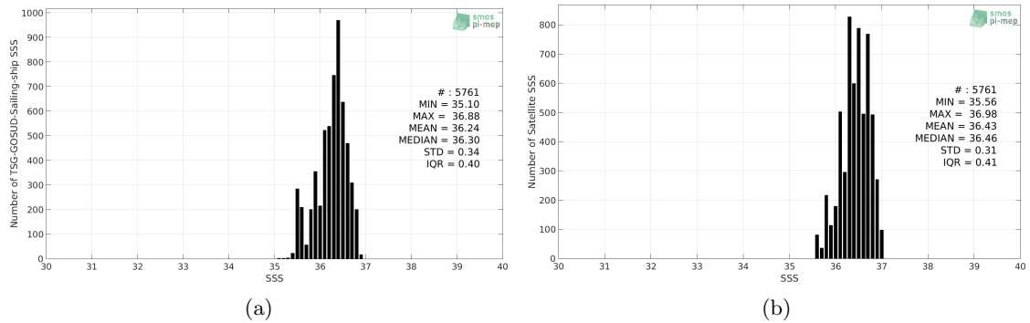
Figure 2: Histograms of SSS from TSG-GOSUD-Sailing-ship (a) and SMAP-L3-RSS-V4-8DAY-RUNNING (b) considering all match-up pairs per bins of 0.1 over the Tropical Atlantic Ocean Pi-MEP region and for the full satellite product period.
