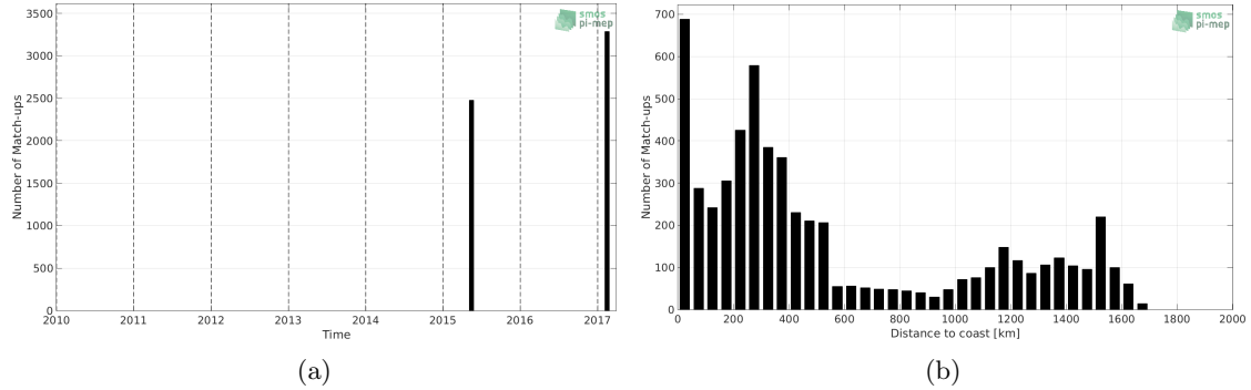
Figure 1: Number of match-ups between TSG-GOSUD-Sailing-ship and SMAP-L3-RSS-V4-8DAY-RUNNING SSS as a function of time (a) and as function of the distance to coast (b) over the Tropical Atlantic Ocean Pi-MEP region and for the full satellite product period.
