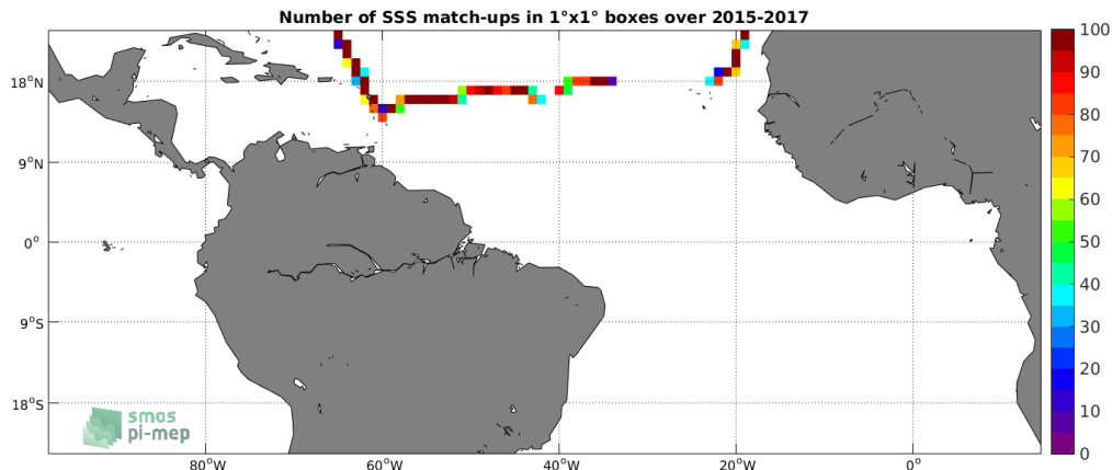
Figure 4: Number of SSS match-ups between TSG-GOSUD-Sailing-ship SSS and the SMAP-L3-RSS-V4-8DAY-RUNNING SSS product for the Tropical Atlantic Ocean Pi-MEP region over 1°x1° boxes and for the full satellite product period.
