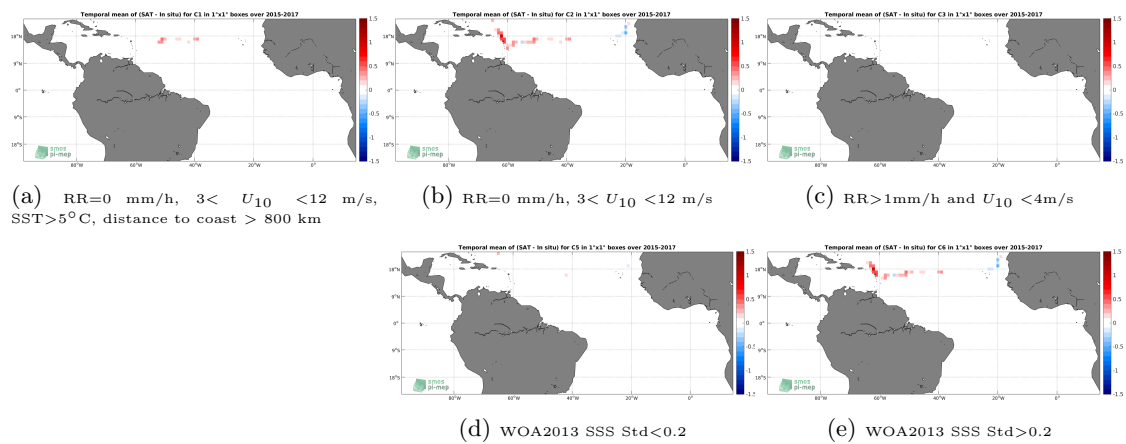
Figure 12: Temporal mean gridded over spatial boxes of size 1^\circ \times 1^\circ of \Delta SSS (SMAP-L3-RSS-V4-8DAY-RUNNING - TSG-GOSUD-Sailing-ship) for 5 different subdatasets corresponding to:RR=0 mm/h, 3 < U_{10} < 12 m/s, SST >5^\circ\text{C} , distance to coast > 800 km (a), RR=0 mm/h, 3 < U_{10} < 12 m/s (b), RR >1 mm/h and U_{10} < 4 m/s (c), WOA2013 SSS Std <0.2 (d), WOA2013 SSS Std >0.2 (e).
