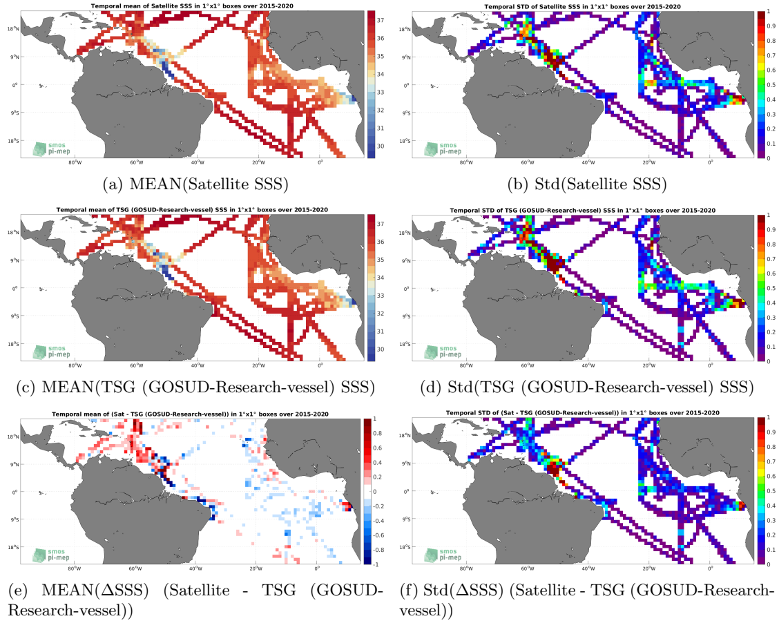
Figure 6: Temporal mean (left) and Std (right) of SSS from SMAP SSS L3 v4 - 8-Day running (RSS) (top), TSG (GOSUD-Research-vessel) (middle), and of \Delta SSS (Satellite - TSG (GOSUD-Research-vessel)). Only match-up pairs are used to generate these maps.
