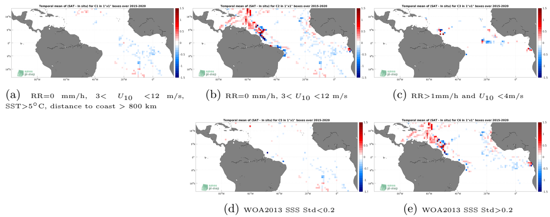
Figure 12: Temporal mean gridded over spatial boxes of size 1^\circ \times 1^\circ of \Delta SSS (SMAP SSS L3 v4 - 8-Day running (RSS) - TSG (GOSUD-Research-vessel)) for 5 different subdatasets corresponding to:RR=0 mm/h, 3 < U_{10} < 12 m/s, SST>5°C, distance to coast > 800 km (a), RR=0 mm/h, 3 < U_{10} < 12 m/s (b), RR>1mm/h and U_{10} < 4 m/s (c), WOA2013 SSS Std<0.2 (d), WOA2013 SSS Std>0.2 (e).
