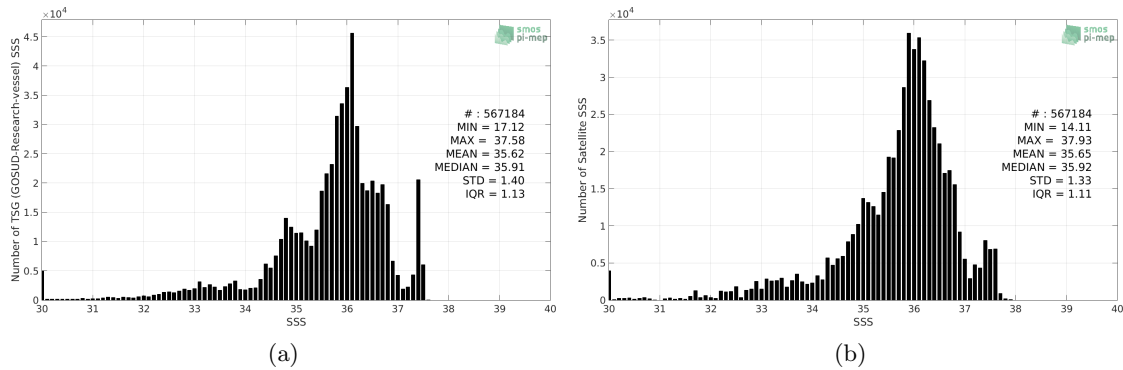
Figure 2: Histograms of SSS from TSG (GOSUD-Research-vessel) (a) and SMAP SSS L3 v4 - 8-Day running (RSS) (b) considering all match-up pairs per bins of 0.1 over the Tropical Atlantic Ocean Pi-MEP region and for the full satellite product period.
