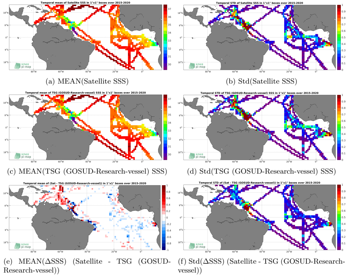
Figure 6: Temporal mean (left) and Std (right) of SSS from SMAP SSS L3 v4 - 8-Day running (RSS) (top), TSG (GOSUD-Research-vessel) (middle), and of \Delta SSS (Satellite - TSG (GOSUD-Research-vessel)). Only match-up pairs are used to generate these maps.
