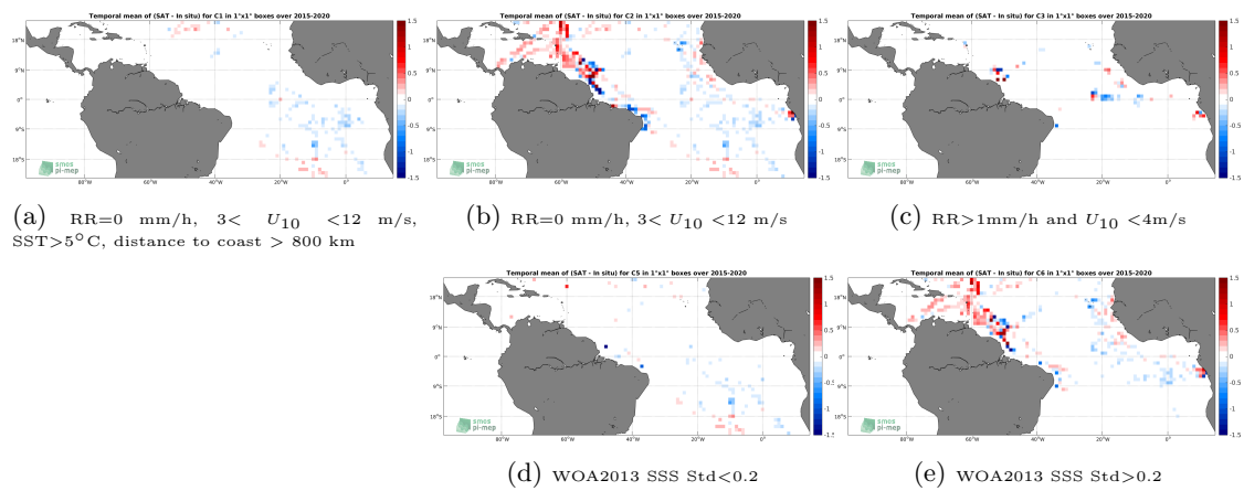
Figure 12: Temporal mean gridded over spatial boxes of size 1^\circ \times 1^\circ of \Delta\text{SSS} (SMAP SSS L3 v4 - 8-Day running (RSS) - TSG (GOSUD-Research-vessel)) for 5 different subdatasets corresponding to:RR=0 mm/h, 3 < U_{10} < 12 m/s, SST>5°C, distance to coast > 800 km (a), RR=0 mm/h, 3 < U_{10} < 12 m/s (b), RR>1mm/h and U_{10} < 4 m/s (c), WOA2013 SSS Std<0.2 (d), WOA2013 SSS Std>0.2 (e).
