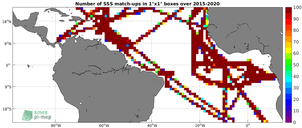
Figure 4: Number of SSS match-ups between TSG (GOSUD-Research-vessel) SSS and the SMAP SSS L3 v4 - 8-Day running (RSS) SSS product for the Tropical Atlantic Ocean Pi-MEP region over 1^\circ \times 1^\circ boxes and for the full satellite product period.
