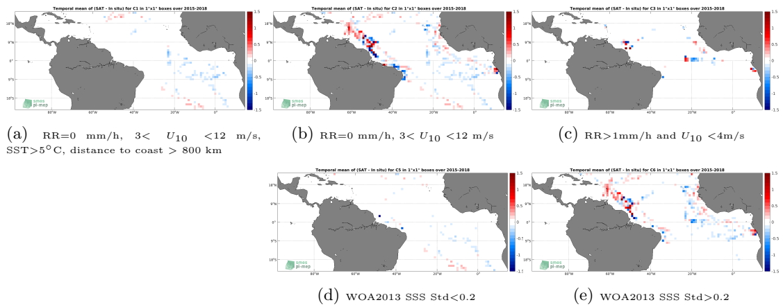
Figure 12: Temporal mean gridded over spatial boxes of size 1°x1° of \Delta SSS (SMAP SSS L3 v4 - 8-Day running (RSS) - TSG (GOSUD-Research-vessel)) for 5 different subdatasets corresponding to:RR=0 mm/h, 3 < U_{10} < 12 m/s, SST>5°C, distance to coast > 800 km (a), RR=0 mm/h, 3 < U_{10} < 12 m/s (b), RR>1mm/h and U_{10} < 4 m/s (c), WOA2013 SSS Std<0.2 (d), WOA2013 SSS Std>0.2 (e).
