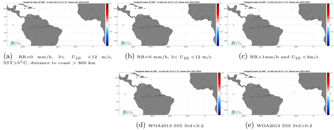
Figure 11: Temporal mean gridded over spatial boxes of size 1^{\circ}\times 1^{\circ} of \Delta\text{SSS} (SMAP SSS L3 v4 - 8-Day running (RSS) - Surface drifters) for 5 different subdatasets corresponding to:RR=0 mm/h, 3 < U_{10} < 12 m/s, SST >5^{\circ}\text{C} , distance to coast > 800 km (a), RR=0 mm/h, 3 < U_{10} < 12 m/s (b), RR >1 mm/h and U_{10} < 4 m/s (c), WOA2013 SSS Std <0.2 (d), WOA2013 SSS Std >0.2 (e).
