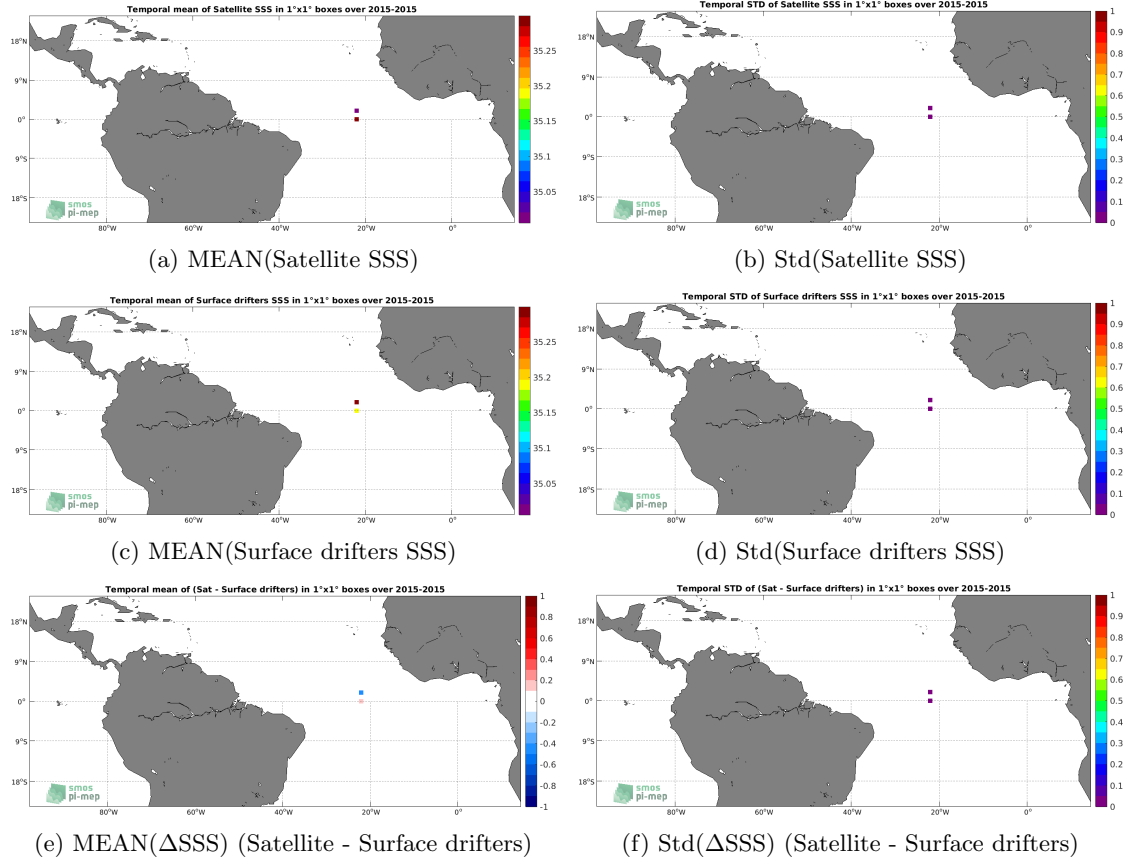
Figure 5: Temporal mean (left) and Std (right) of SSS from SMAP SSS L3 v4 - 8-Day running (RSS) (top), Surface drifters (middle), and of \Delta SSS (Satellite - Surface drifters). Only match-up pairs are used to generate these maps.
