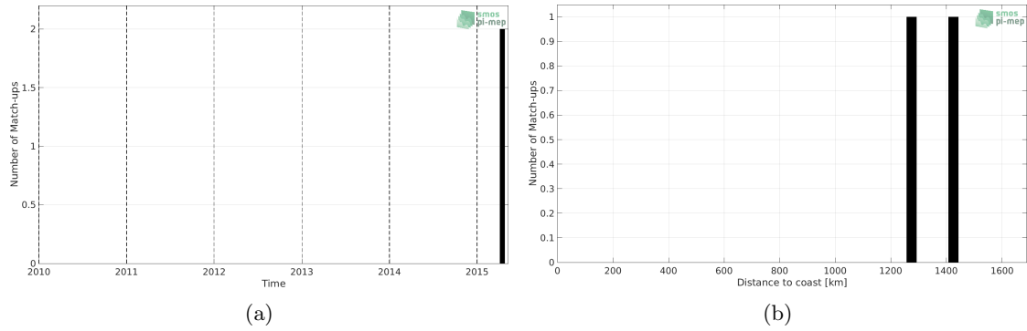
Figure 1: Number of match-ups between Surface drifters and SMAP SSS L3 v4 - 8-Day running (RSS) SSS as a function of time (a) and as function of the distance to coast (b) over the Tropical Atlantic Ocean Pi-MEP region and for the full satellite product period.
