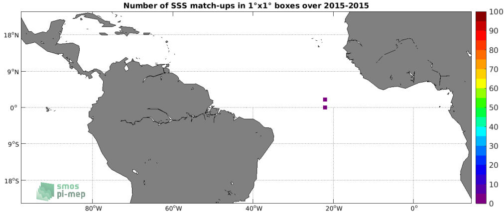
Figure 3: Number of SSS match-ups between Surface drifters SSS and the SMAP SSS L3 v4 - 8-Day running (RSS) SSS product for the Tropical Atlantic Ocean Pi-MEP region over 1^\circ \times 1^\circ boxes and for the full satellite product period.
