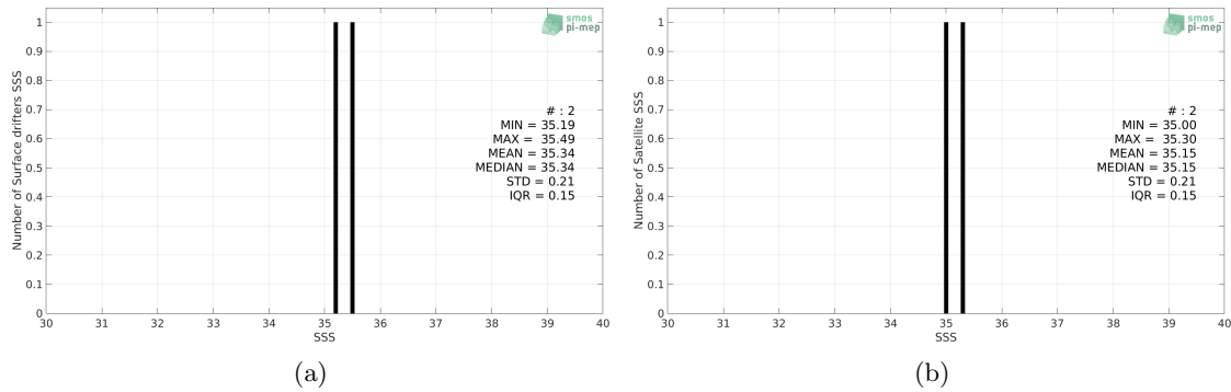
Figure 2: Histograms of SSS from Surface drifters (a) and SMAP SSS L3 v4 - 8-Day running (RSS) (b) considering all match-up pairs per bins of 0.1 over the Tropical Atlantic Ocean Pi-MEP region and for the full satellite product period.
