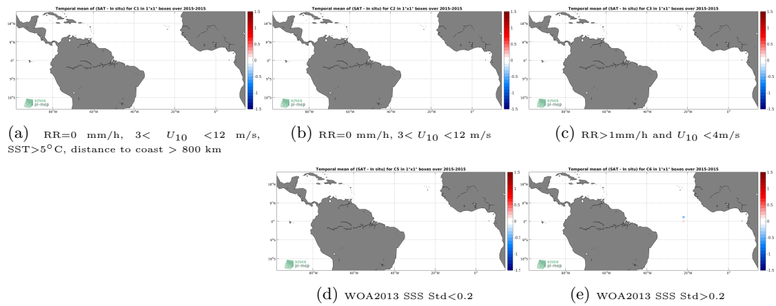
Figure 11: Temporal mean gridded over spatial boxes of size 1^\circ \times 1^\circ of \Delta SSS (SMAP-L3-RSS-V4-8DAY-RUNNING - Surface drifters) for 5 different subdatasets corresponding to:RR=0 mm/h, 3 < U_{10} < 12 m/s, SST >5^\circ C, distance to coast > 800 km (a), RR=0 mm/h, 3 < U_{10} < 12 m/s (b), RR >1 mm/h and U_{10} < 4 m/s (c), WOA2013 SSS Std <0.2 (d), WOA2013 SSS Std >0.2 (e).
