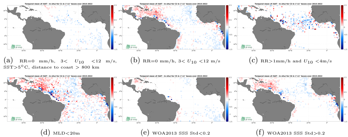
Figure 12: Temporal mean gridded over spatial boxes of size 1^\circ \times 1^\circ of \Delta SSS (SMAP SSS L3 v4 - 8-Day running (RSS) - Argo) for 6 different subdatasets corresponding to:RR=0 mm/h, 3 < U_{10} < 12 m/s, SST >5^\circ C, distance to coast > 800 km (a), RR=0 mm/h, 3 < U_{10} < 12 m/s (b), RR >1 mm/h and U_{10} < 4 m/s (c),MLD <20 m (d),WOA2013 SSS Std <0.2 (e),WOA2013 SSS Std >0.2 (f).
