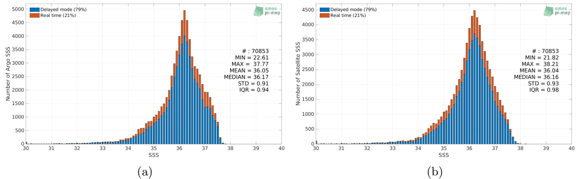
Figure 2: Histograms of SSS from Argo (a) and SMAP SSS L3 v4 - 8-Day running (RSS) (b) considering all match-up pairs per bins of 0.1 over the Tropical Atlantic Ocean Pi-MEP region and for the full satellite product period.
