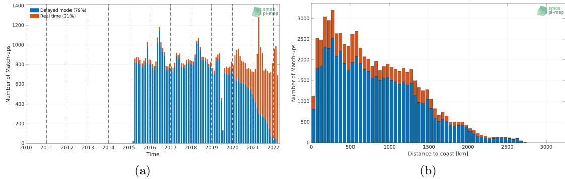
Figure 1: Number of match-ups between Argo and SMAP SSS L3 v4 - 8-Day running (RSS) SSS as a function of time (a) and as function of the distance to coast (b) over the Tropical Atlantic Ocean Pi-MEP region and for the full satellite product period.
