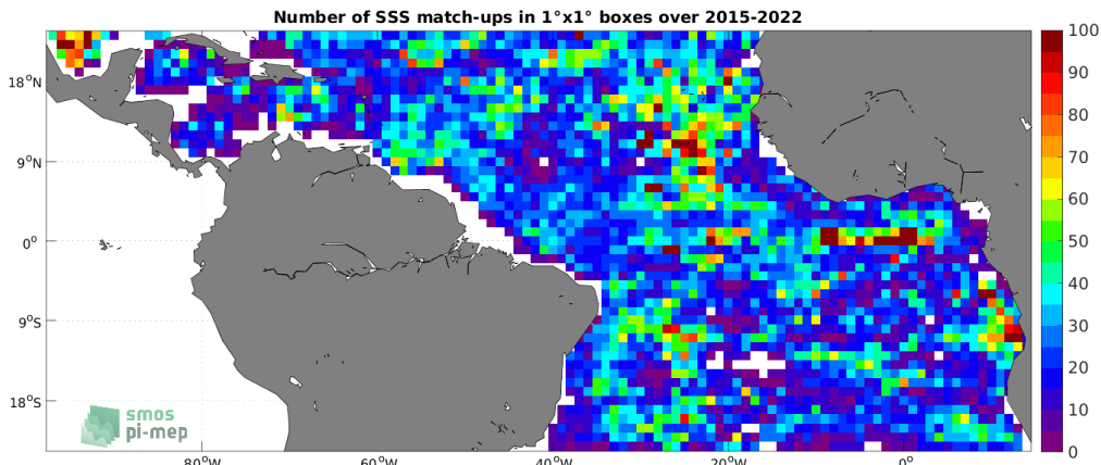
Figure 4: Number of SSS match-ups between Argo SSS and the SMAP SSS L3 v4 - 8-Day running (RSS) SSS product for the Tropical Atlantic Ocean Pi-MEP region over 1^\circ \times 1^\circ boxes and for the full satellite product period.
