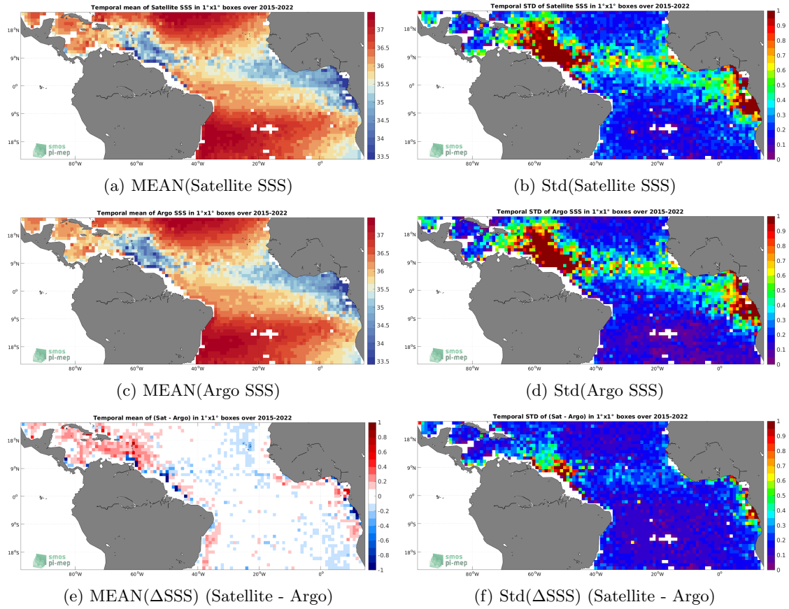
Figure 6: Temporal mean (left) and Std (right) of SSS from SMAP SSS L3 v4 - 8-Day running (RSS) (top), Argo (middle), and of \Delta SSS (Satellite - Argo). Only match-up pairs are used to generate these maps.
