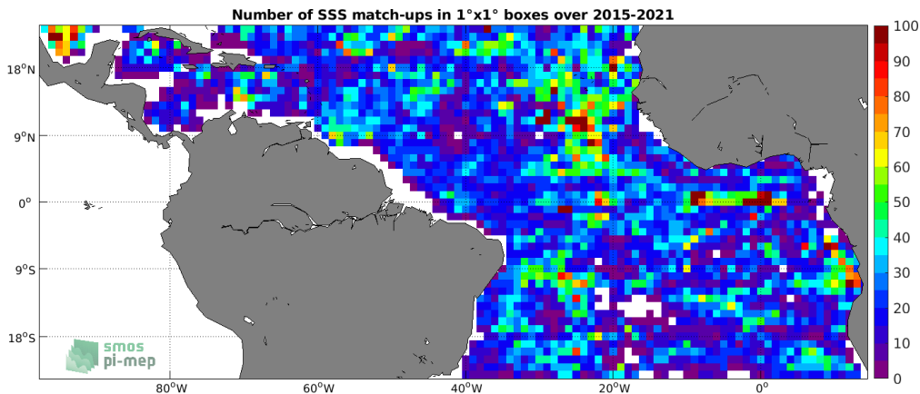
Figure 4: Number of SSS match-ups between Argo SSS and the SMAP SSS L3 v4 - 8-Day running (RSS) SSS product for the Tropical Atlantic Ocean Pi-MEP region over 1°x1° boxes and for the full satellite product period.
