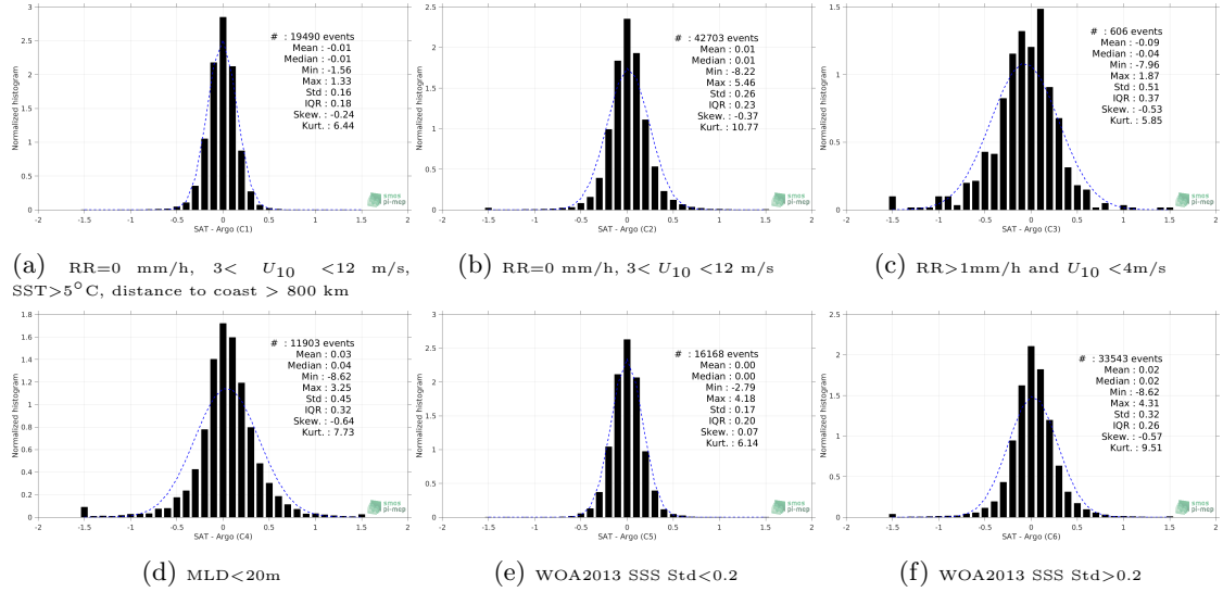
Figure 13: Normalized histogram of \Delta\text{SSS} (SMAP-L3-RSS-V4-8DAY-RUNNING - Argo) for 6 different subdatasets corresponding to: RR=0 mm/h, 3 < U_{10} < 12 m/s, SST>5°C, distance to coast > 800 km (a), RR=0 mm/h, 3 < U_{10} < 12 m/s (b), RR>1mm/h and U_{10} < 4 m/s (c), MLD<20m (d), WOA2013 SSS Std<0.2 (e), WOA2013 SSS Std>0.2 (f).
