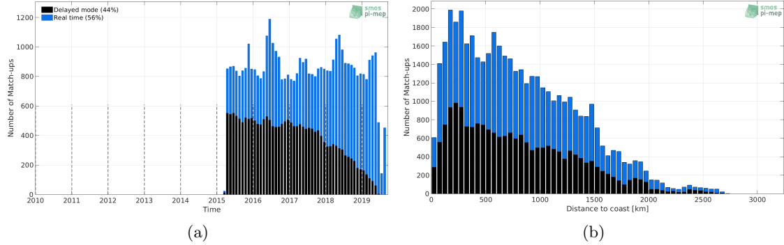
Figure 1: Number of match-ups between Argo and SMAP-L3-RSS-V4-8DAY-RUNNING SSS as a function of time (a) and as function of the distance to coast (b) over the Tropical Atlantic Ocean Pi-MEP region and for the full satellite product period.
