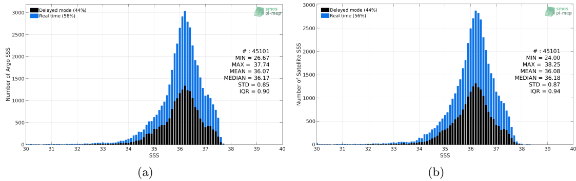
Figure 2: Histograms of SSS from Argo (a) and SMAP-L3-RSS-V4-8DAY-RUNNING (b) considering all match-up pairs per bins of 0.1 over the Tropical Atlantic Ocean Pi-MEP region and for the full satellite product period.
