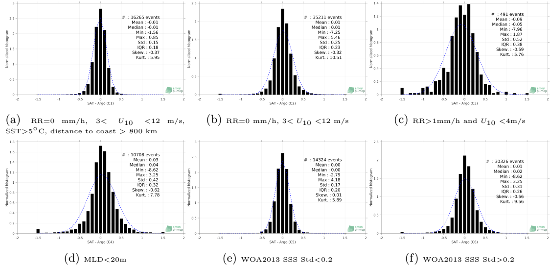
Figure 13: Normalized histogram of \Delta\text{SSS} (SMAP-L3-RSS-V4-8DAY-RUNNING - Argo) for 6 different subdatasets corresponding to: RR=0 mm/h, 3 < U_{10} < 12 m/s, SST>5°C, distance to coast > 800 km (a), RR=0 mm/h, 3 < U_{10} < 12 m/s (b), RR>1mm/h and U_{10} < 4 m/s (c), MLD<20m (d), WOA2013 SSS Std<0.2 (e), WOA2013 SSS Std>0.2 (f).
