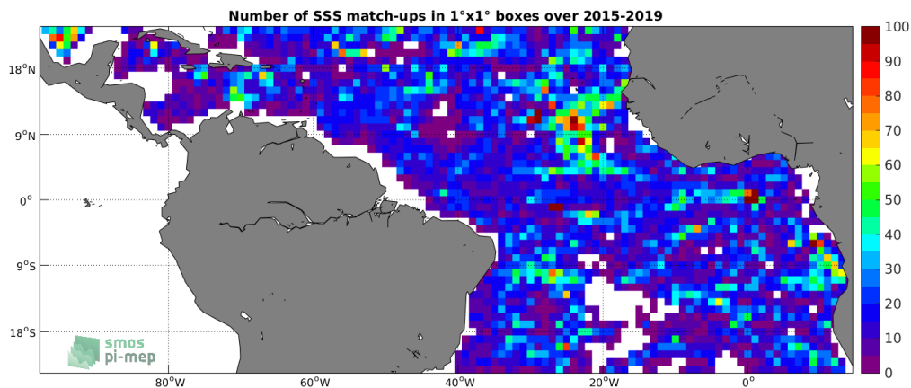
Figure 4: Number of SSS match-ups between Argo SSS and the SMAP-L3-RSS-V4-8DAY-RUNNING SSS product for the Tropical Atlantic Ocean Pi-MEP region over 1°x1° boxes and for the full satellite product period.
