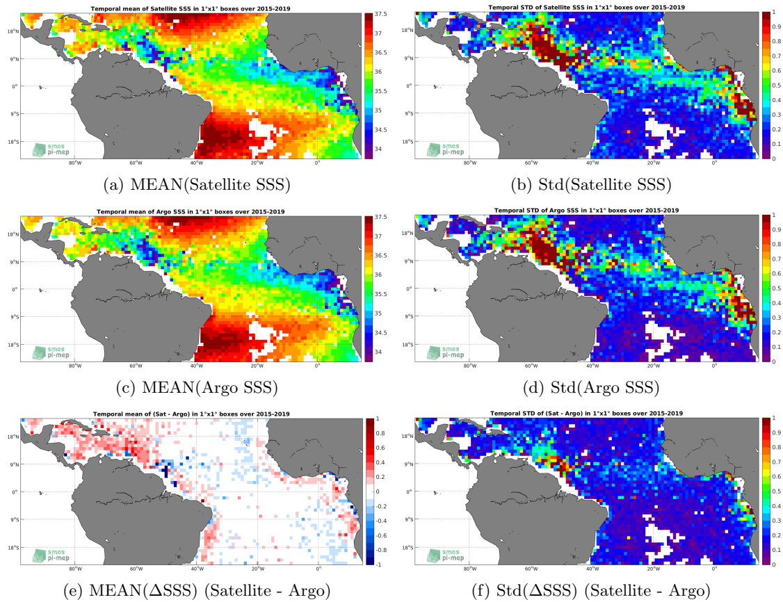
Figure 6: Temporal mean (left) and Std (right) of SSS from SMAP-L3-RSS-V4-8DAY-RUNNING (top), Argo (middle), and of \Delta SSS (Satellite - Argo). Only match-up pairs are used to generate these maps.
