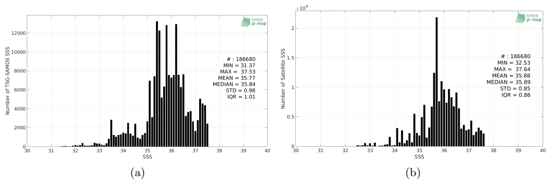
Figure 2: Histograms of SSS from TSG-SAMOS (a) and SMAP-L3-RSS-V4-MONTHLY (b) considering all match-up pairs per bins of 0.1 over the Tropical Atlantic Ocean Pi-MEP region and for the full satellite product period.
