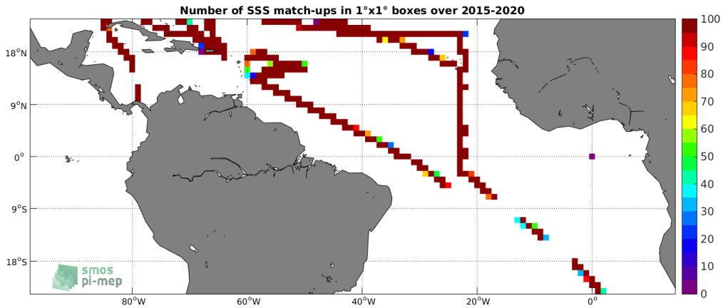
Figure 4: Number of SSS match-ups between TSG-SAMOS SSS and the SMAP-L3-RSS-V4-MONTHLY SSS product for the Tropical Atlantic Ocean Pi-MEP region over 1^\circ \times 1^\circ boxes and for the full satellite product period.
