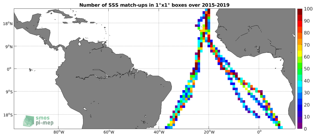
Figure 4: Number of SSS match-ups between TSG (Polarstern) SSS and the SMAP SSS L3 v4 - Monthly (RSS) SSS product for the Tropical Atlantic Ocean Pi-MEP region over 1°x1° boxes and for the full satellite product period.
