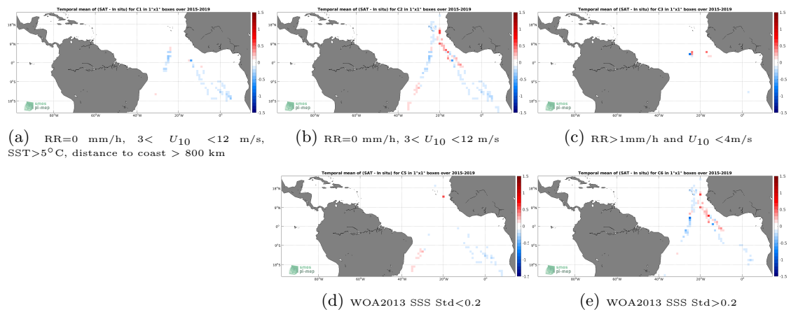
Figure 12: Temporal mean gridded over spatial boxes of size 1^\circ \times 1^\circ of \Delta SSS (SMAP SSS L3 v4 - Monthly (RSS) - TSG (Polarstern)) for 5 different subdatasets corresponding to: RR=0 mm/h, 3 < U_{10} < 12 m/s, SST > 5°C, distance to coast > 800 km (a), RR=0 mm/h, 3 < U_{10} < 12 m/s (b), RR > 1mm/h and U_{10} < 4 m/s (c), WOA2013 SSS Std < 0.2 (d), WOA2013 SSS Std > 0.2 (e).
