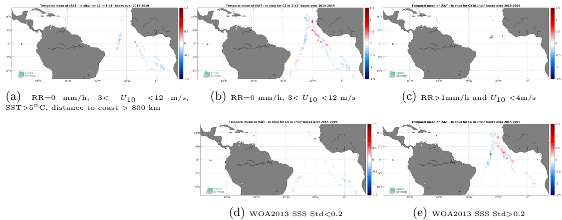
Figure 12: Temporal mean gridded over spatial boxes of size 1^\circ \times 1^\circ of \Delta SSS (SMAP-L3-RSS-V4-MONTHLY - TSG-POLARSTERN) for 5 different subdatasets corresponding to:RR=0 mm/h, 3 < U_{10} < 12 m/s, SST >5^\circ\text{C} , distance to coast > 800 km (a), RR=0 mm/h, 3 < U_{10} < 12 m/s (b), RR >1 mm/h and U_{10} < 4 m/s (c), WOA2013 SSS Std <0.2 (d), WOA2013 SSS Std >0.2 (e).
