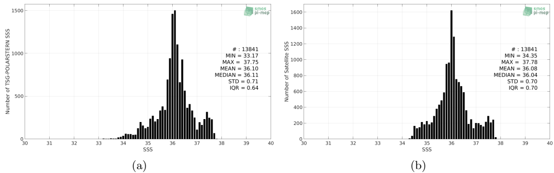
Figure 2: Histograms of SSS from TSG-POLARSTERN (a) and SMAP-L3-RSS-V4-MONTHLY (b) considering all match-up pairs per bins of 0.1 over the Tropical Atlantic Ocean Pi-MEP region and for the full satellite product period.
