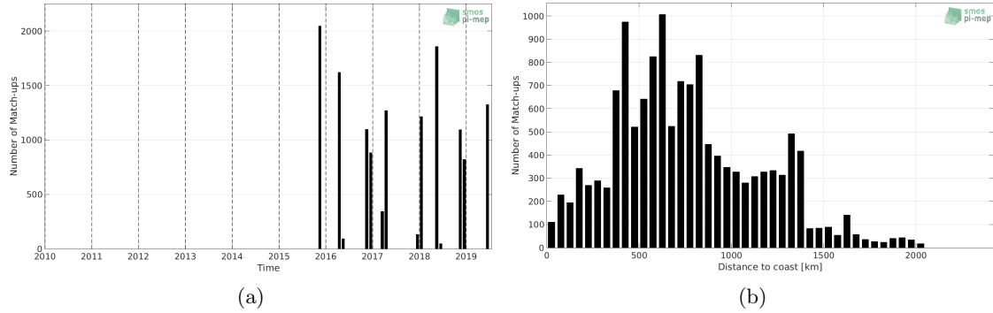
Figure 1: Number of match-ups between TSG-POLARSTERN and SMAP-L3-RSS-V4-MONTHLY SSS as a function of time (a) and as function of the distance to coast (b) over the Tropical Atlantic Ocean Pi-MEP region and for the full satellite product period.
