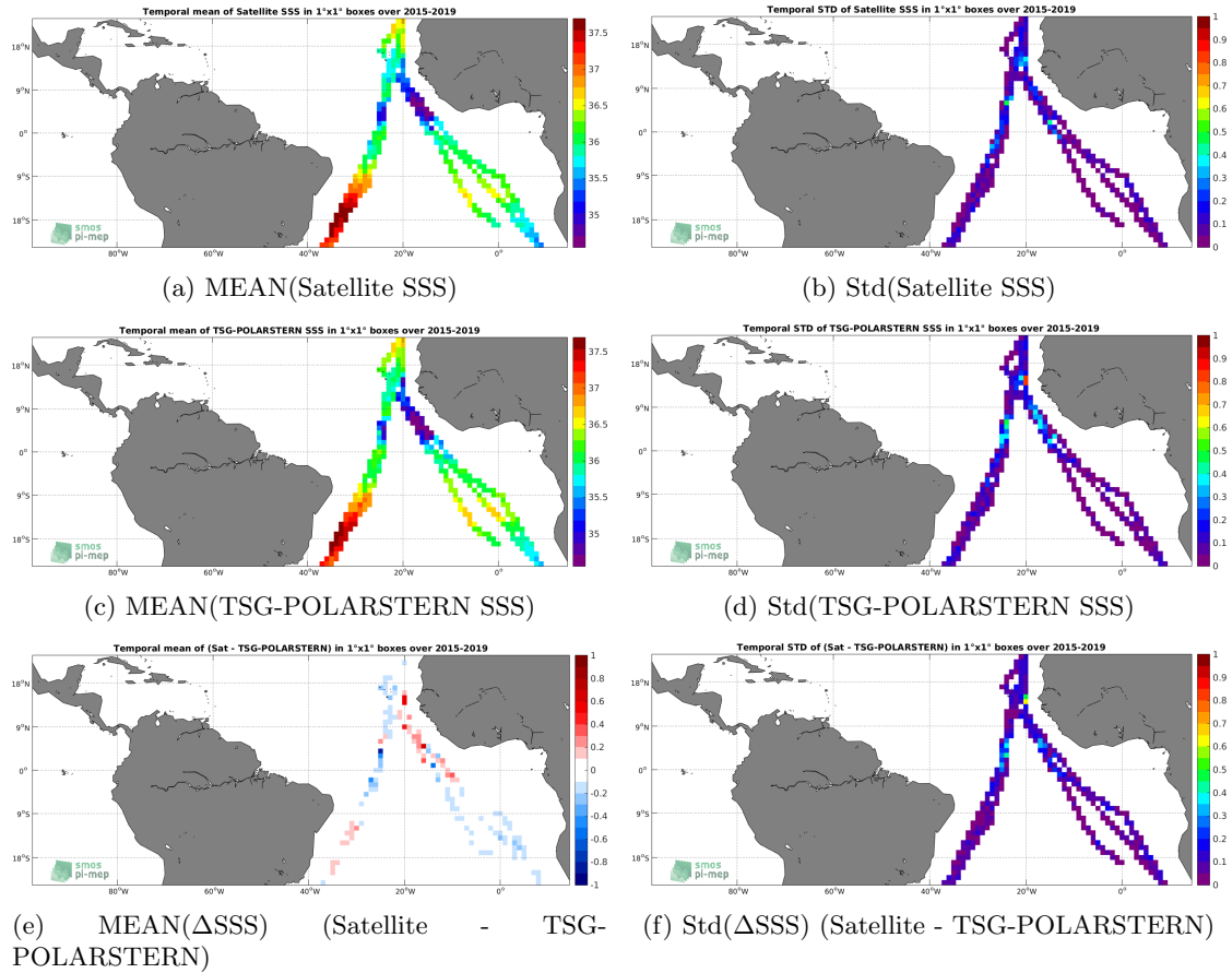
Figure 6: Temporal mean (left) and Std (right) of SSS from SMAP-L3-RSS-V4-MONTHLY (top), TSG-POLARSTERN (middle), and of \Delta SSS (Satellite - TSG-POLARSTERN). Only match-up pairs are used to generate these maps.
