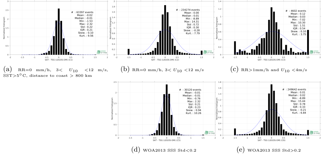
Figure 13: Normalized histogram of \Delta SSS (SMAP SSS L3 v4 - Monthly (RSS) - TSG (LEGOS-DMI)) for 5 different subdatasets corresponding to: RR=0 mm/h, 3 < U_{10} < 12 m/s, SST > 5°C, distance to coast > 800 km (a), RR=0 mm/h, 3 < U_{10} < 12 m/s (b), RR > 1mm/h and U_{10} < 4 m/s (c), WOA2013 SSS Std < 0.2 (d), WOA2013 SSS Std > 0.2 (e).
