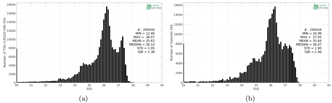
Figure 2: Histograms of SSS from TSG (LEGOS-DM) (a) and SMAP SSS L3 v4 - Monthly (RSS) (b) considering all match-up pairs per bins of 0.1 over the Tropical Atlantic Ocean Pi-MEP region and for the full satellite product period.
