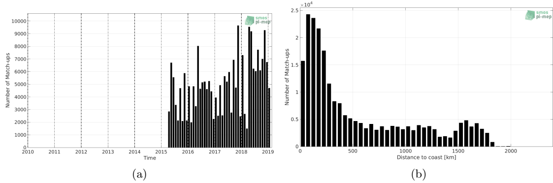
Figure 1: Number of match-ups between TSG (LEGOS-DM) and SMAP SSS L3 v4 - Monthly (RSS) SSS as a function of time (a) and as function of the distance to coast (b) over the Tropical Atlantic Ocean Pi-MEP region and for the full satellite product period.
