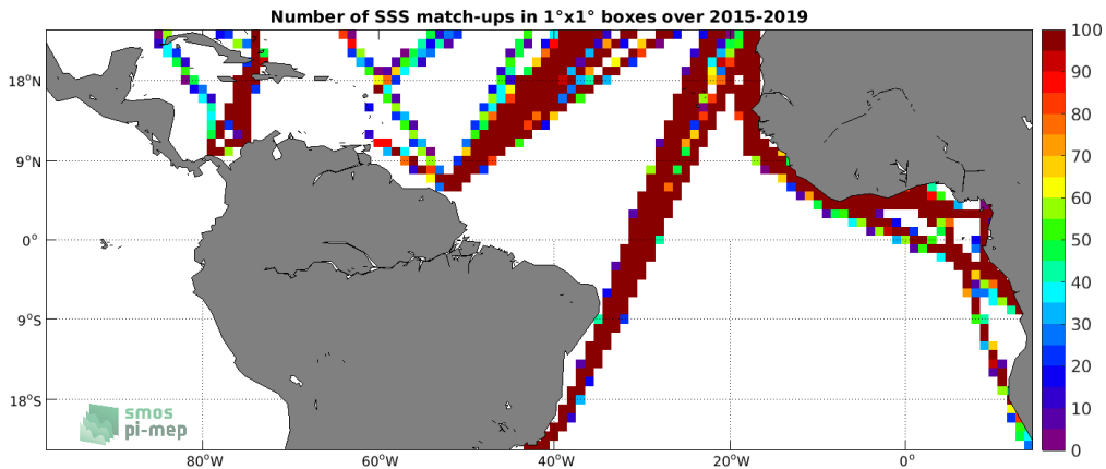
Figure 4: Number of SSS match-ups between TSG (LEGOS-DM) SSS and the SMAP SSS L3 v4 - Monthly (RSS) SSS product for the Tropical Atlantic Ocean Pi-MEP region over 1^\circ \times 1^\circ boxes and for the full satellite product period.
