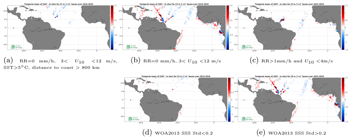
Figure 12: Temporal mean gridded over spatial boxes of size 1°x1° of \Delta SSS (SMAP SSS L3 v4 - Monthly (RSS) - TSG (LEGOS-DM)) for 5 different subdatasets corresponding to:RR=0 mm/h, 3 < U_{10} < 12 m/s, SST>5°C, distance to coast > 800 km (a), RR=0 mm/h, 3 < U_{10} < 12 m/s (b), RR>1mm/h and U_{10} < 4 m/s (c), WOA2013 SSS Std<0.2 (d), WOA2013 SSS Std>0.2 (e).
