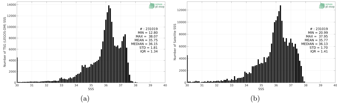
Figure 2: Histograms of SSS from TSG (LEGOS-DM) (a) and SMAP SSS L3 v4 - Monthly (RSS) (b) considering all match-up pairs per bins of 0.1 over the Tropical Atlantic Ocean Pi-MEP region and for the full satellite product period.
