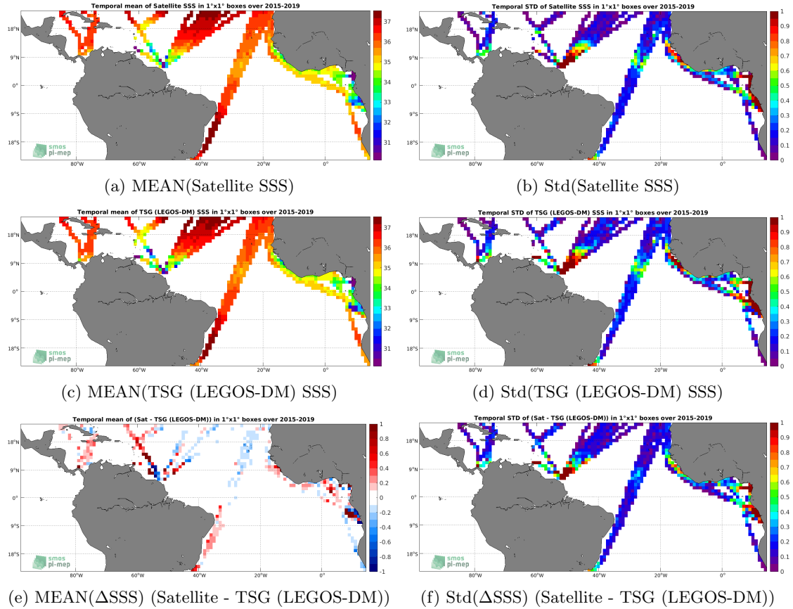
Figure 6: Temporal mean (left) and Std (right) of SSS from SMAP SSS L3 v4 - Monthly (RSS) (top), TSG (LEGOS-DM) (middle), and of \Delta SSS (Satellite - TSG (LEGOS-DM)). Only match-up pairs are used to generate these maps.
