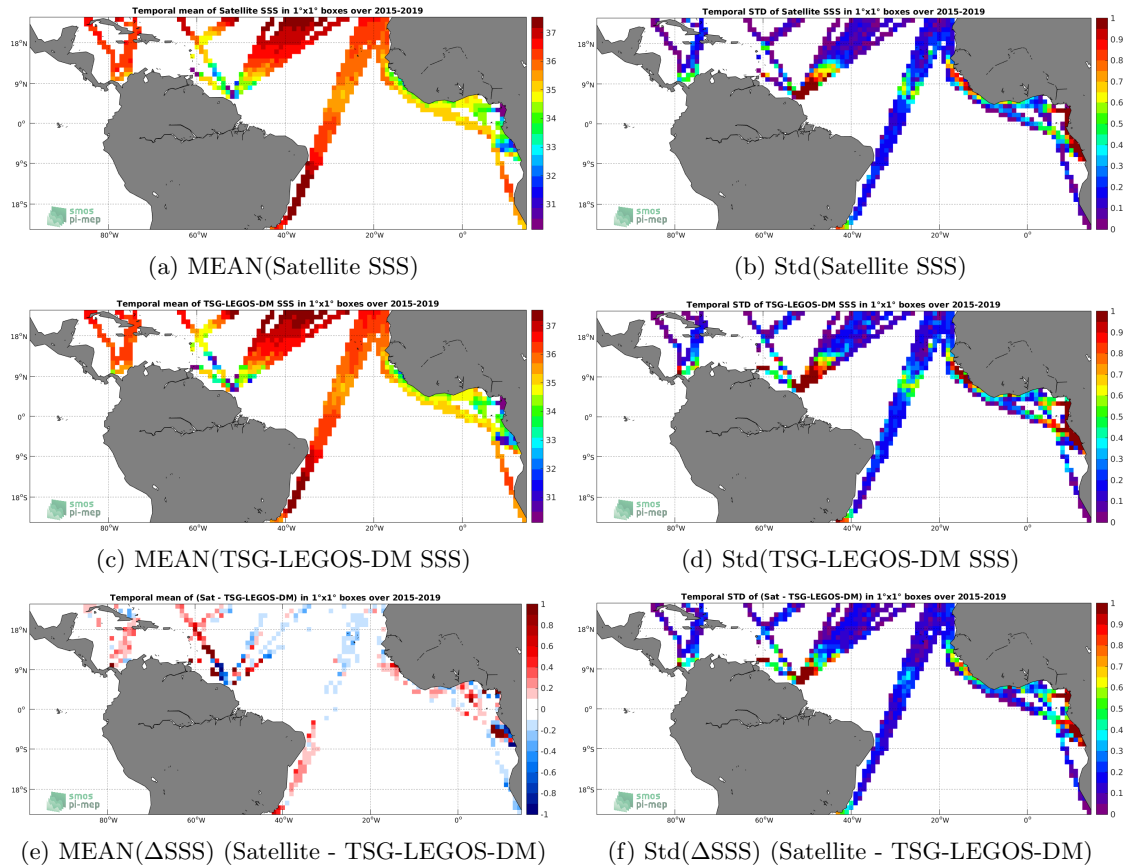
Figure 6: Temporal mean (left) and Std (right) of SSS from SMAP-L3-RSS-V4-MONTHLY (top), TSG-LEGOS-DM (middle), and of \Delta SSS (Satellite - TSG-LEGOS-DM). Only match-up pairs are used to generate these maps.
