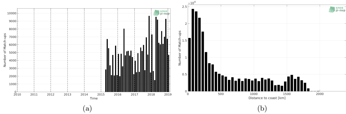
Figure 1: Number of match-ups between TSG-LEGOS-DM and SMAP-L3-RSS-V4-MONTHLY SSS as a function of time (a) and as function of the distance to coast (b) over the Tropical Atlantic Ocean Pi-MEP region and for the full satellite product period.
