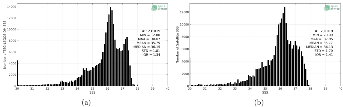
Figure 2: Histograms of SSS from TSG-LEGOS-DM (a) and SMAP-L3-RSS-V4-MONTHLY (b) considering all match-up pairs per bins of 0.1 over the Tropical Atlantic Ocean Pi-MEP region and for the full satellite product period.
