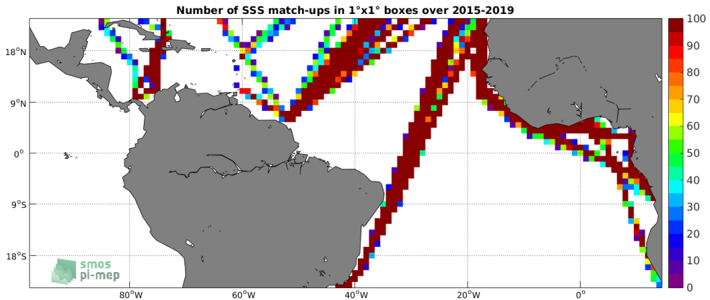
Figure 4: Number of SSS match-ups between TSG-LEGOS-DM SSS and the SMAP-L3-RSS-V4-MONTHLY SSS product for the Tropical Atlantic Ocean Pi-MEP region over 1^\circ \times 1^\circ boxes and for the full satellite product period.
