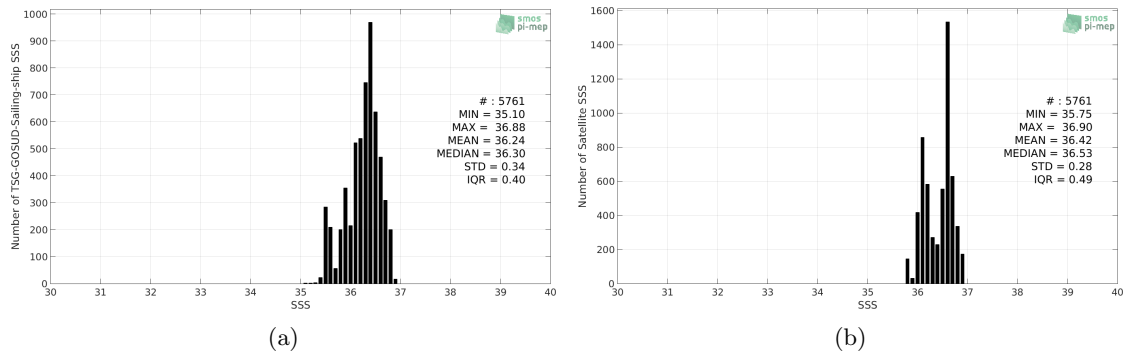
Figure 2: Histograms of SSS from TSG-GOSUD-Sailing-ship (a) and SMAP-L3-RSS-V4-MONTHLY (b) considering all match-up pairs per bins of 0.1 over the Tropical Atlantic Ocean Pi-MEP region and for the full satellite product period.
