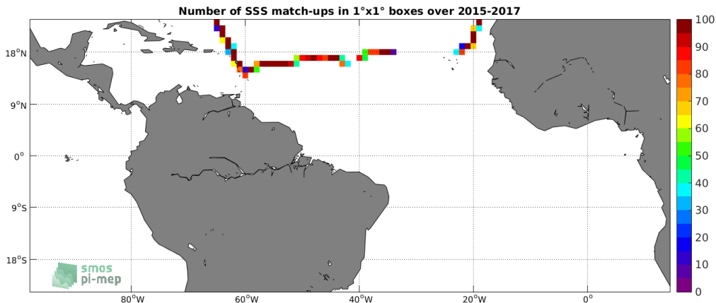
Figure 4: Number of SSS match-ups between TSG-GOSUD-Sailing-ship SSS and the SMAP-L3-RSS-V4-MONTHLY SSS product for the Tropical Atlantic Ocean Pi-MEP region over 1°x1° boxes and for the full satellite product period.
