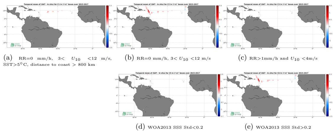
Figure 12: Temporal mean gridded over spatial boxes of size 1^\circ \times 1^\circ of \Delta SSS (SMAP-L3-RSS-V4-MONTHLY - TSG-GOSUD-Sailing-ship) for 5 different subdatasets corresponding to:RR=0 mm/h, 3 < U_{10} < 12 m/s, SST >5^\circ\text{C} , distance to coast > 800 km (a), RR=0 mm/h, 3 < U_{10} < 12 m/s (b), RR >1 mm/h and U_{10} < 4 m/s (c), WOA2013 SSS Std <0.2 (d), WOA2013 SSS Std >0.2 (e).
