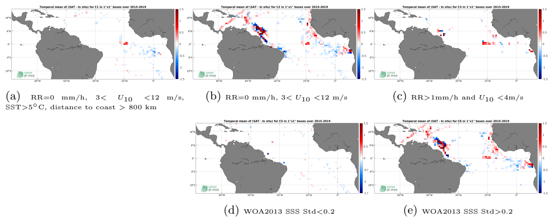
Figure 12: Temporal mean gridded over spatial boxes of size 1^\circ \times 1^\circ of \Delta\text{SSS} (SMAP SSS L3 v4 - Monthly (RSS) - TSG (GOSUD-Research-vessel)) for 5 different subdatasets corresponding to: RR=0 mm/h, 3 < U_{10} < 12 m/s, SST > 5°C, distance to coast > 800 km (a), RR=0 mm/h, 3 < U_{10} < 12 m/s (b), RR > 1mm/h and U_{10} < 4 m/s (c), WOA2013 SSS Std < 0.2 (d), WOA2013 SSS Std > 0.2 (e).
