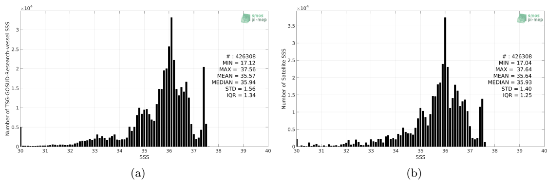
Figure 2: Histograms of SSS from TSG-GOSUD-Research-vessel (a) and SMAP-L3-RSS-V4-MONTHLY (b) considering all match-up pairs per bins of 0.1 over the Tropical Atlantic Ocean Pi-MEP region and for the full satellite product period.
