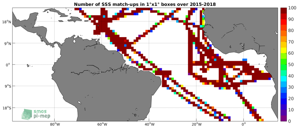
Figure 4: Number of SSS match-ups between TSG-GOSUD-Research-vessel SSS and the SMAP-L3-RSS-V4-MONTHLY SSS product for the Tropical Atlantic Ocean Pi-MEP region over 1^\circ \times 1^\circ boxes and for the full satellite product period.
