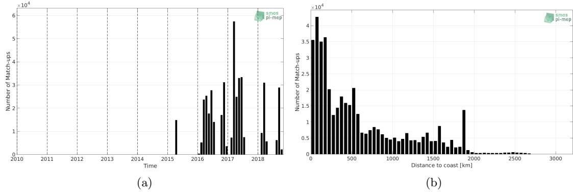
Figure 1: Number of match-ups between TSG-GOSUD-Research-vessel and SMAP-L3-RSS-V4-MONTHLY SSS as a function of time (a) and as function of the distance to coast (b) over the Tropical Atlantic Ocean Pi-MEP region and for the full satellite product period.
