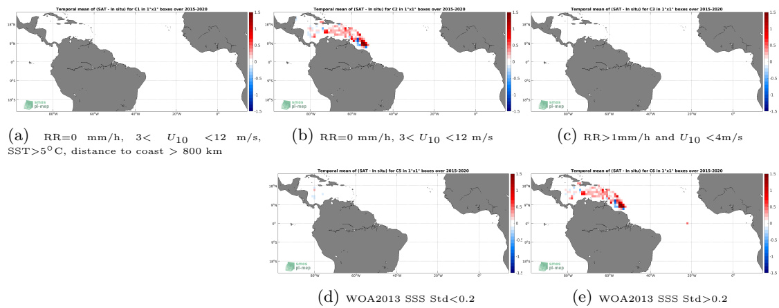
Figure 11: Temporal mean gridded over spatial boxes of size 1^\circ \times 1^\circ of \Delta SSS (SMAP SSS L3 v4 - Monthly (RSS) - Surface drifters) for 5 different subdatasets corresponding to: RR=0 mm/h, 3 < U_{10} < 12 m/s, SST > 5^\circ\text{C} , distance to coast > 800 km (a), RR=0 mm/h, 3 < U_{10} < 12 m/s (b), RR > 1 mm/h and U_{10} < 4 m/s (c), WOA2013 SSS Std < 0.2 (d), WOA2013 SSS Std > 0.2 (e).
