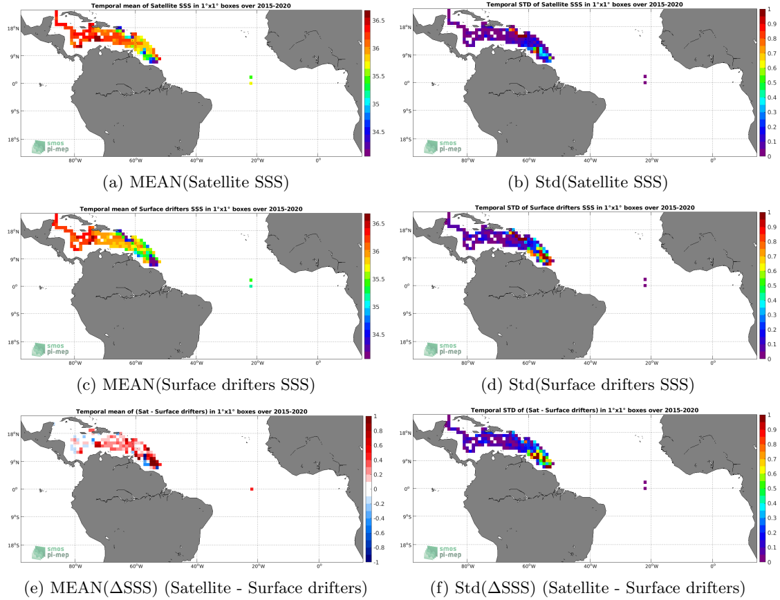
Figure 5: Temporal mean (left) and Std (right) of SSS from SMAP SSS L3 v4 - Monthly (RSS) (top), Surface drifters (middle), and of \Delta SSS (Satellite - Surface drifters). Only match-up pairs are used to generate these maps.
