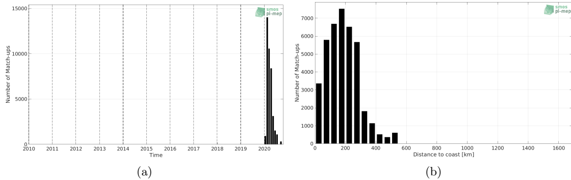
Figure 1: Number of match-ups between Surface drifters and SMAP SSS L3 v4 - Monthly (RSS) SSS as a function of time (a) and as function of the distance to coast (b) over the Tropical Atlantic Ocean Pi-MEP region and for the full satellite product period.
