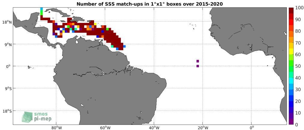
Figure 3: Number of SSS match-ups between Surface drifters SSS and the SMAP SSS L3 v4 - Monthly (RSS) SSS product for the Tropical Atlantic Ocean Pi-MEP region over 1^\circ \times 1^\circ boxes and for the full satellite product period.
