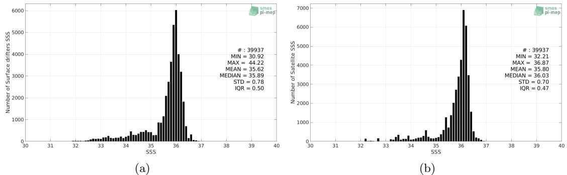
Figure 2: Histograms of SSS from Surface drifters (a) and SMAP SSS L3 v4 - Monthly (RSS) (b) considering all match-up pairs per bins of 0.1 over the Tropical Atlantic Ocean Pi-MEP region and for the full satellite product period.
