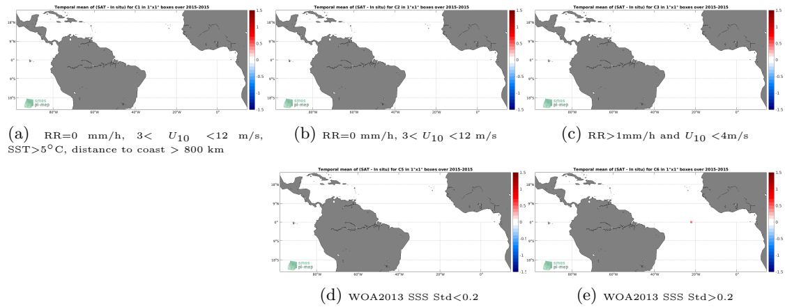
Figure 11: Temporal mean gridded over spatial boxes of size 1^{\circ}\times 1^{\circ} of \Delta\text{SSS} (SMAP SSS L3 v4 - Monthly (RSS) - Surface drifters) for 5 different subdatasets corresponding to:RR=0 mm/h, 3 < U_{10} < 12 m/s, SST >5^{\circ}\text{C} , distance to coast > 800 km (a), RR=0 mm/h, 3 < U_{10} < 12 m/s (b), RR >1 mm/h and U_{10} < 4 m/s (c), WOA2013 SSS Std <0.2 (d), WOA2013 SSS Std >0.2 (e).
