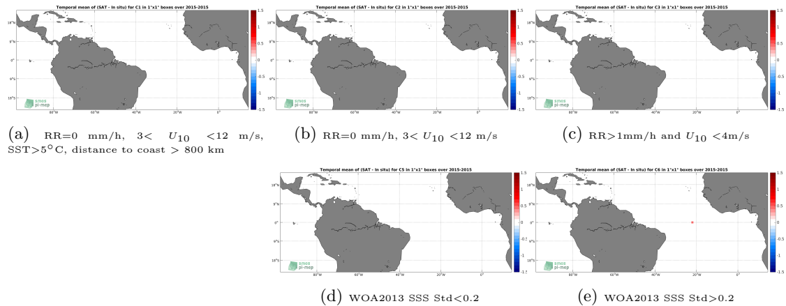
Figure 11: Temporal mean gridded over spatial boxes of size 1^{\circ}\times 1^{\circ} of \Delta\text{SSS} (SMAP-L3-RSS-V4-MONTHLY - Surface drifters) for 5 different subdatasets corresponding to:RR=0 mm/h, 3 < U_{10} < 12 m/s, SST > 5^{\circ}\text{C} , distance to coast > 800 km (a), RR=0 mm/h, 3 < U_{10} < 12 m/s (b), RR > 1 mm/h and U_{10} < 4 m/s (c), WOA2013 SSS Std < 0.2 (d), WOA2013 SSS Std > 0.2 (e).
