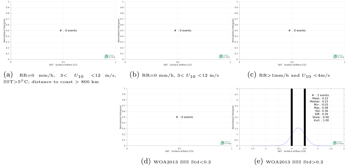
Figure 12: Normalized histogram of \Delta\text{SSS} (SMAP-L3-RSS-V4-MONTHLY - Surface drifters) for 5 different subdatasets corresponding to: RR=0 mm/h, 3 < U_{10} < 12 m/s, SST > 5^\circ\text{C} , distance to coast > 800 km (a), RR=0 mm/h, 3 < U_{10} < 12 m/s (b), RR > 1\text{mm/h} and U_{10} < 4\text{m/s} (c), WOA2013 SSS Std < 0.2 (d), WOA2013 SSS Std > 0.2 (e).
