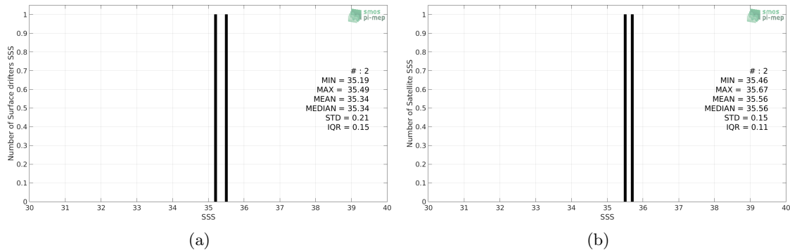
Figure 2: Histograms of SSS from Surface drifters (a) and SMAP-L3-RSS-V4-MONTHLY (b) considering all match-up pairs per bins of 0.1 over the Tropical Atlantic Ocean Pi-MEP region and for the full satellite product period.
