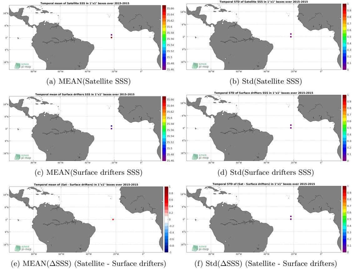
Figure 5: Temporal mean (left) and Std (right) of SSS from SMAP-L3-RSS-V4-MONTHLY (top), Surface drifters (middle), and of \Delta SSS (Satellite - Surface drifters). Only match-up pairs are used to generate these maps.
