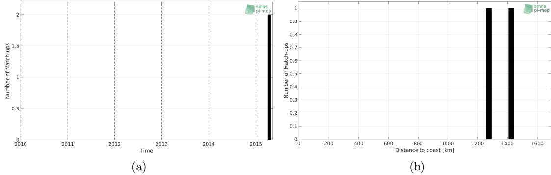
Figure 1: Number of match-ups between Surface drifters and SMAP-L3-RSS-V4-MONTHLY SSS as a function of time (a) and as function of the distance to coast (b) over the Tropical Atlantic Ocean Pi-MEP region and for the full satellite product period.
