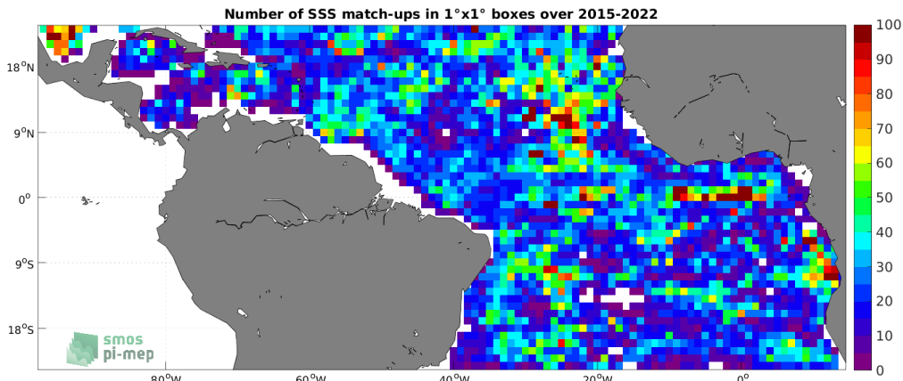
Figure 4: Number of SSS match-ups between Argo SSS and the SMAP SSS L3 v4 - Monthly (RSS) SSS product for the Tropical Atlantic Ocean Pi-MEP region over 1^\circ \times 1^\circ boxes and for the full satellite product period.
