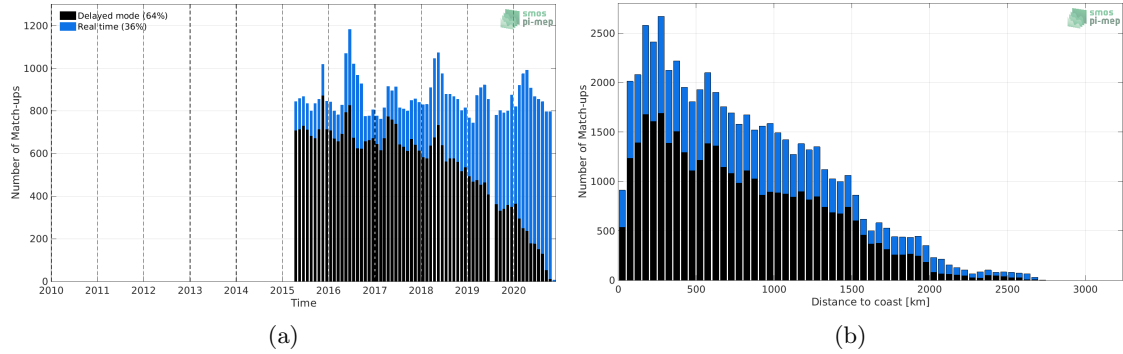
Figure 1: Number of match-ups between Argo and SMAP SSS L3 v4 - Monthly (RSS) SSS as a function of time (a) and as function of the distance to coast (b) over the Tropical Atlantic Ocean Pi-MEP region and for the full satellite product period.
