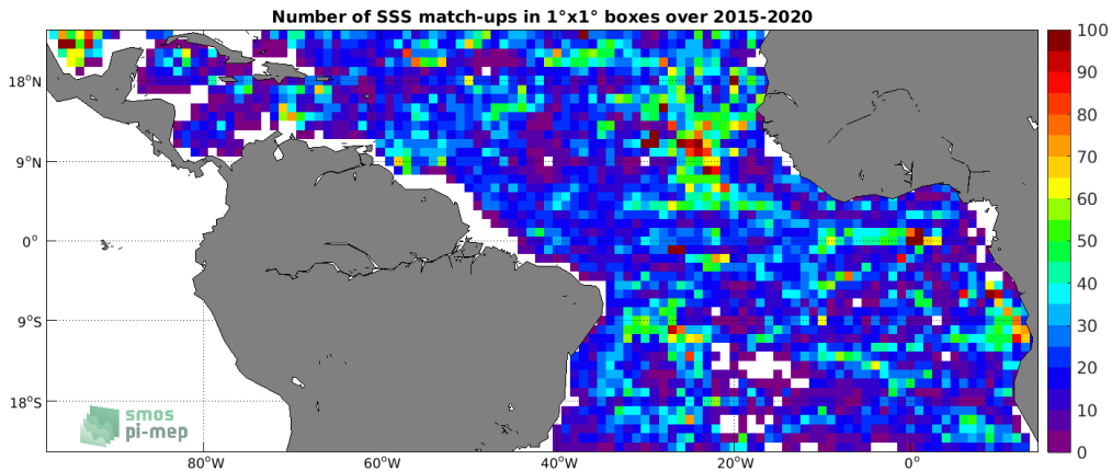
Figure 4: Number of SSS match-ups between Argo SSS and the SMAP SSS L3 v4 - Monthly (RSS) SSS product for the Tropical Atlantic Ocean Pi-MEP region over 1°x1° boxes and for the full satellite product period.
