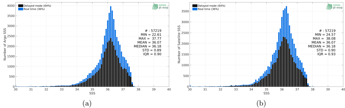
Figure 2: Histograms of SSS from Argo (a) and SMAP SSS L3 v4 - Monthly (RSS) (b) considering all match-up pairs per bins of 0.1 over the Tropical Atlantic Ocean Pi-MEP region and for the full satellite product period.
