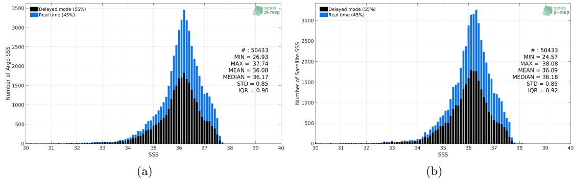
Figure 2: Histograms of SSS from Argo (a) and SMAP-L3-RSS-V4-MONTHLY (b) considering all match-up pairs per bins of 0.1 over the Tropical Atlantic Ocean Pi-MEP region and for the full satellite product period.
