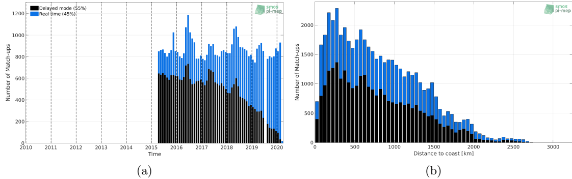
Figure 1: Number of match-ups between Argo and SMAP-L3-RSS-V4-MONTHLY SSS as a function of time (a) and as function of the distance to coast (b) over the Tropical Atlantic Ocean Pi-MEP region and for the full satellite product period.
