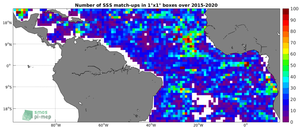
Figure 4: Number of SSS match-ups between Argo SSS and the SMAP-L3-RSS-V4-MONTHLY SSS product for the Tropical Atlantic Ocean Pi-MEP region over 1°x1° boxes and for the full satellite product period.
