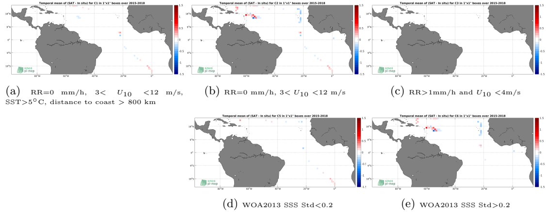
Figure 12: Temporal mean gridded over spatial boxes of size 1^\circ \times 1^\circ of \Delta SSS (SMAP-L3-RSS-V3-8DAY-RUNNING-70KM - TSG-SAMOS) for 5 different subdatasets corresponding to: RR=0 mm/h, 3 < U_{10} < 12 m/s, SST > 5^\circ C , distance to coast > 800 km (a), RR=0 mm/h, 3 < U_{10} < 12 m/s (b), RR > 1 mm/h and U_{10} < 4 m/s (c), WOA2013 SSS Std < 0.2 (d), WOA2013 SSS Std > 0.2 (e).
