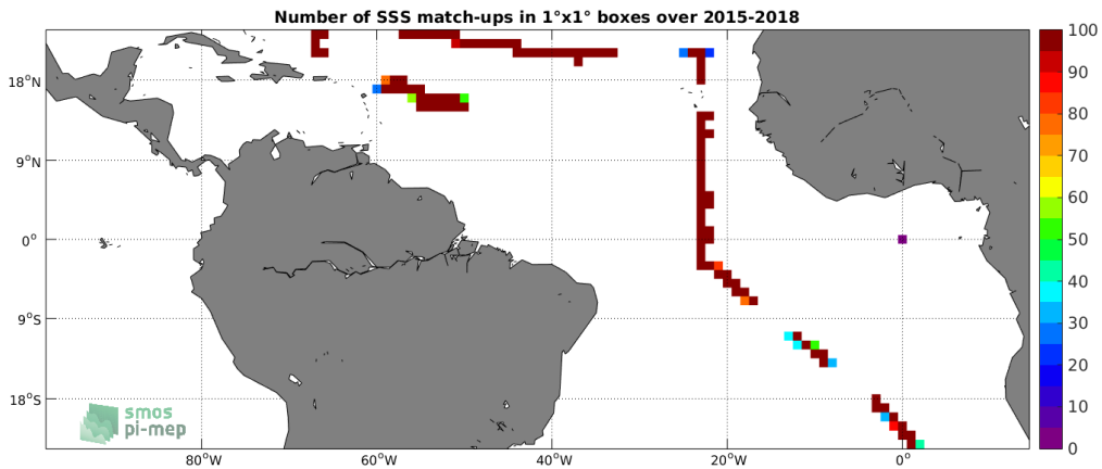
Figure 4: Number of SSS match-ups between TSG-SAMOS SSS and the SMAP-L3-RSS-V3-8DAY-RUNNING-70KM SSS product for the Tropical Atlantic Ocean Pi-MEP region over 1^\circ \times 1^\circ boxes and for the full satellite product period.
