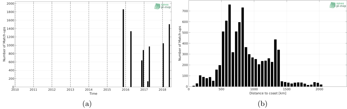
Figure 1: Number of match-ups between TSG-POLARSTERN and SMAP-L3-RSS-V3-8DAY-RUNNING-70KM SSS as a function of time (a) and as function of the distance to coast (b) over the Tropical Atlantic Ocean Pi-MEP region and for the full satellite product period.
