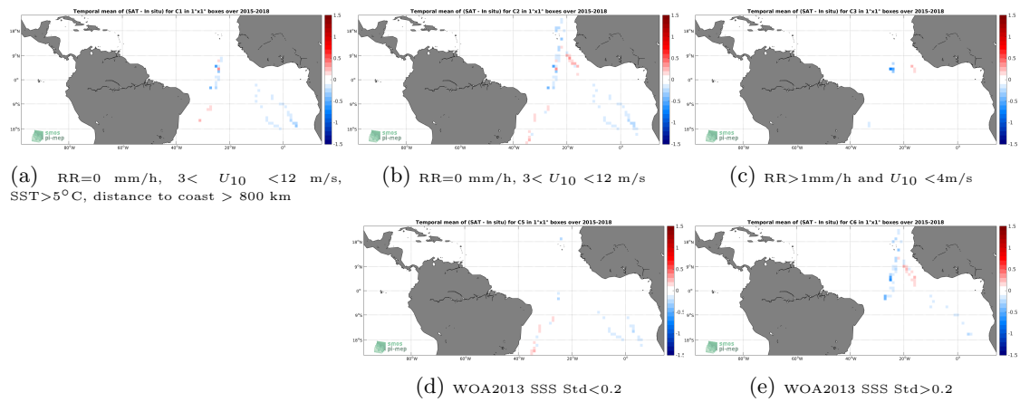
Figure 12: Temporal mean gridded over spatial boxes of size 1^\circ \times 1^\circ of \Delta SSS (SMAP-L3-RSS-V3-8DAY-RUNNING-70KM - TSG-POLARSTERN) for 5 different subdatasets corresponding to:RR=0 mm/h, 3 < U_{10} < 12 m/s, SST >5^\circ C, distance to coast > 800 km (a), RR=0 mm/h, 3 < U_{10} < 12 m/s (b), RR >1 mm/h and U_{10} < 4 m/s (c), WOA2013 SSS Std <0.2 (d), WOA2013 SSS Std >0.2 (e).
