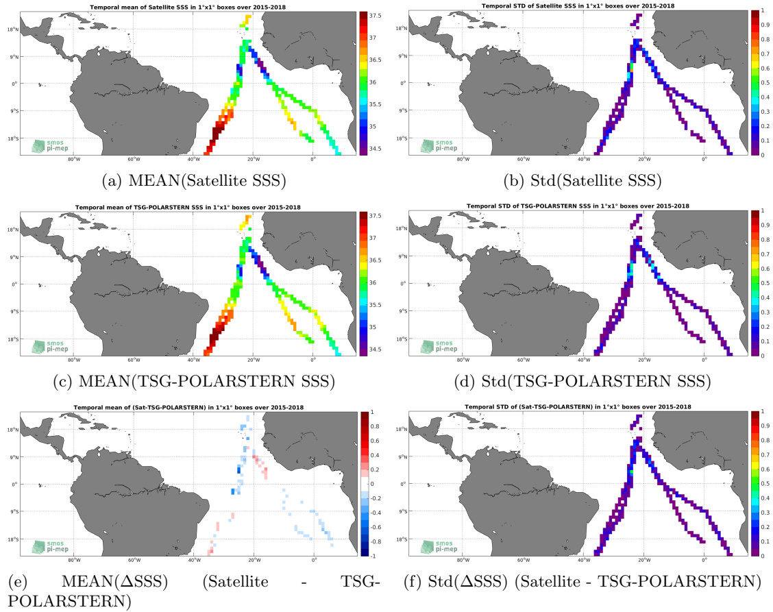
Figure 6: Temporal mean (left) and Std (right) of SSS from SMAP-L3-RSS-V3-8DAY-RUNNING-70KM (top), TSG-POLARSTERN (middle), and of \Delta SSS (Satellite - TSG-POLARSTERN). Only match-up pairs are used to generate these maps.
