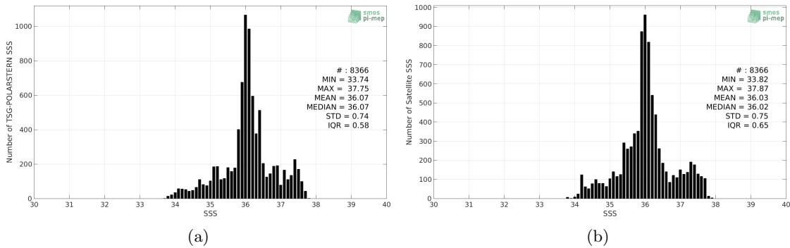
Figure 2: Histograms of SSS from TSG-POLARSTERN (a) and SMAP-L3-RSS-V3-8DAY-RUNNING-70KM (b) considering all match-up pairs per bins of 0.1 over the Tropical Atlantic Ocean Pi-MEP region and for the full satellite product period.
