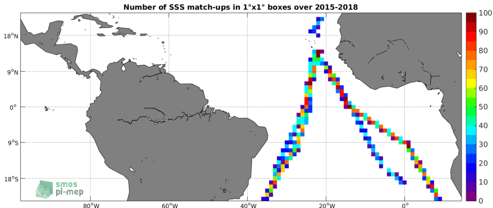
Figure 4: Number of SSS match-ups between TSG-POLARSTERN SSS and the SMAP-L3-RSS-V3-8DAY-RUNNING-70KM SSS product for the Tropical Atlantic Ocean Pi-MEP region over 1^\circ \times 1^\circ boxes and for the full satellite product period.
