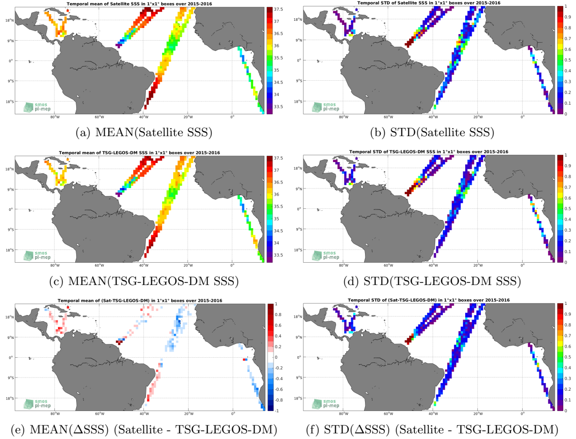
Figure 6: Temporal mean (left) and STD (right) of SSS from SMAP-L3-RSS-V3-8DAY-RUNNING-70KM (top), TSG-LEGOS-DM (middle), and of \Delta SSS (Satellite - TSG-LEGOS-DM). Only match-up pairs are used to generate these maps.
