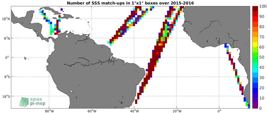
Figure 4: Number of SSS match-ups between TSG-LEGOS-DM SSS and the SMAP-L3-RSS-V3-8DAY-RUNNING-70KM SSS product for the Tropical Atlantic Ocean Pi-MEP region over 1^\circ \times 1^\circ boxes and for the full satellite product period.
