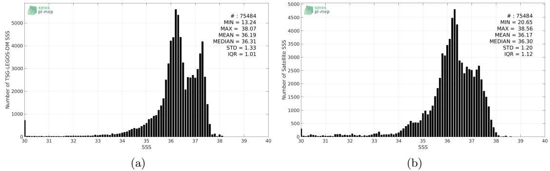
Figure 2: Histograms of SSS from TSG-LEGOS-DM (a) and SMAP-L3-RSS-V3-8DAY-RUNNING-70KM (b) considering all match-up pairs per bins of 0.1 over the Tropical Atlantic Ocean Pi-MEP region and for the full satellite product period.
