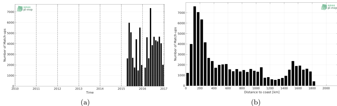
Figure 1: Number of match-ups between TSG-LEGOS-DM and SMAP-L3-RSS-V3-8DAY-RUNNING-70KM SSS as a function of time (a) and as function of the distance to coast (b) over the Tropical Atlantic Ocean Pi-MEP region and for the full satellite product period.
