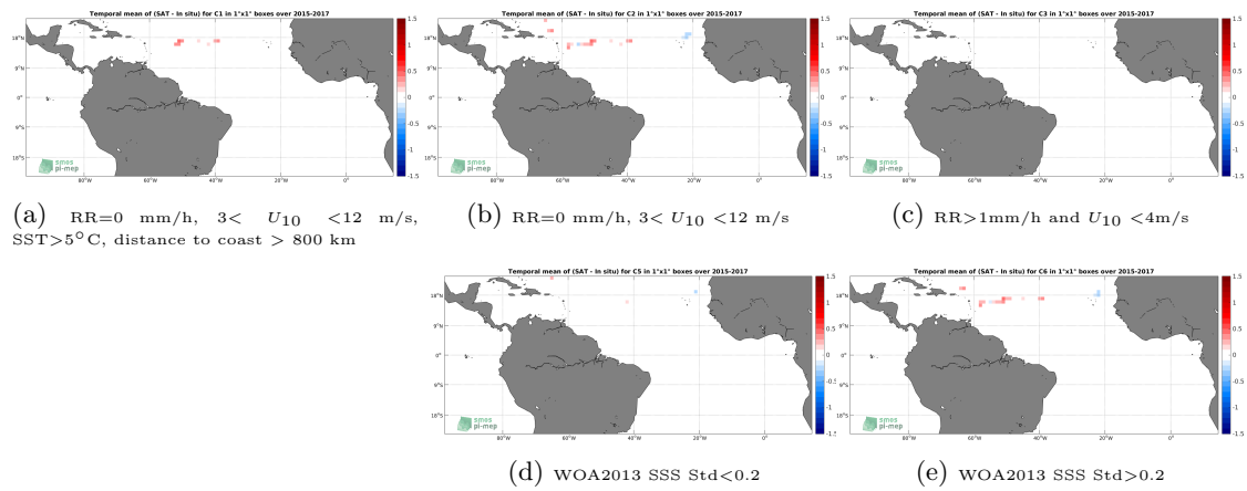
Figure 12: Temporal mean gridded over spatial boxes of size 1^\circ \times 1^\circ of \Delta SSS (SMAP-L3-RSS-V3-8DAY-RUNNING-70KM - TSG-GOSUD-Sailing-ship) for 5 different subdatasets corresponding to:RR=0 mm/h, 3 < U_{10} < 12 m/s, SST >5^\circ C, distance to coast > 800 km (a), RR=0 mm/h, 3 < U_{10} < 12 m/s (b), RR >1 mm/h and U_{10} < 4 m/s (c), WOA2013 SSS Std <0.2 (d), WOA2013 SSS Std >0.2 (e).
