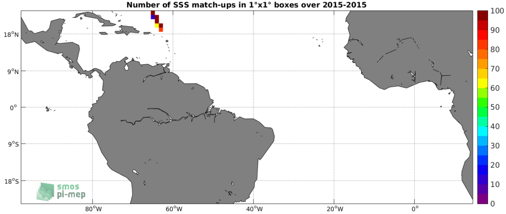
Figure 4: Number of SSS match-ups between TSG-GOSUD-Sailing-ship SSS and the SMAP-L3-RSS-V3-8DAY-RUNNING-70KM SSS product for the Tropical Atlantic Ocean Pi-MEP region over 1^\circ \times 1^\circ boxes and for the full satellite product period.
