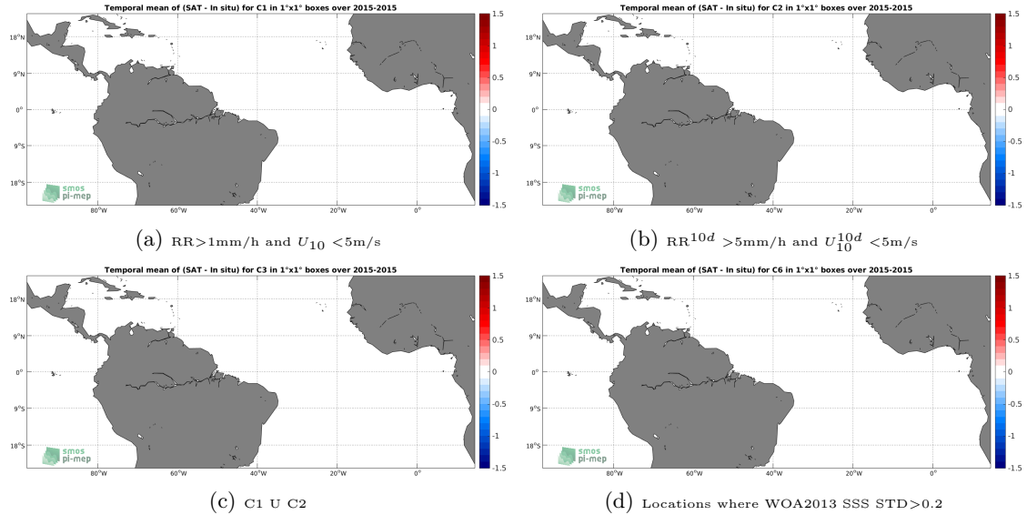
Figure 12: Temporal mean gridded over spatial boxes of size 1^\circ \times 1^\circ of \Delta SSS (SMAP-L3-RSS-V3-8DAY-RUNNING-70KM - TSG-GOSUD-Sailing-ship) for 4 different subdatasets corresponding to:RR > 1 mm/h and U_{10} < 5 m/s (a), RR^{10d} > 5 mm/h and U_{10}^{10d} < 5 m/s (b), C1 U C2 (c),Locations where WOA2013 SSS STD > 0.2 (d).
