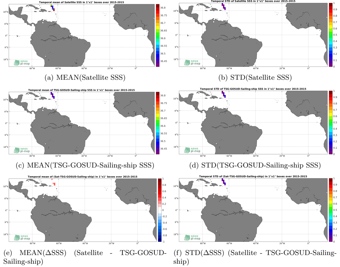
Figure 6: Temporal mean (left) and STD (right) of SSS from SMAP-L3-RSS-V3-8DAY-RUNNING-70KM (top), TSG-GOSUD-Sailing-ship (middle), and of \Delta SSS (Satellite - TSG-GOSUD-Sailing-ship). Only match-up pairs are used to generate these maps.
