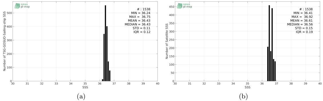
Figure 2: Histograms of SSS from TSG-GOSUD-Sailing-ship (a) and SMAP-L3-RSS-V3-8DAY-RUNNING-70KM (b) considering all match-up pairs per bins of 0.1 over the Tropical Atlantic Ocean Pi-MEP region and for the full satellite product period.
