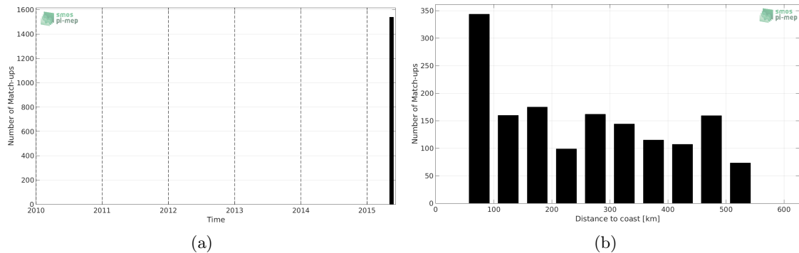
Figure 1: Number of match-ups between TSG-GOSUD-Sailing-ship and SMAP-L3-RSS-V3-8DAY-RUNNING-70KM SSS as a function of time (a) and as function of the distance to coast (b) over the Tropical Atlantic Ocean Pi-MEP region and for the full satellite product period.
