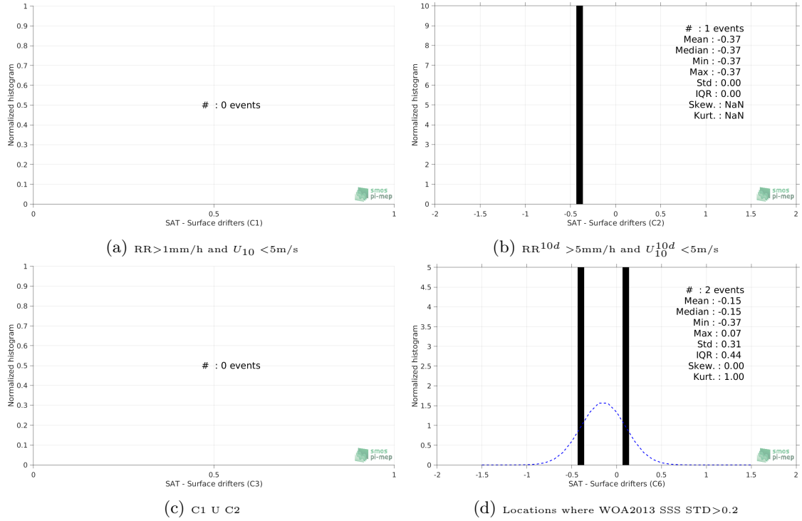
Figure 12: Normalized histogram of \Delta\text{SSS} (SMAP-L3-RSS-V3-8DAY-RUNNING-70KM - Surface drifters) for 6 different subdatasets corresponding to: RR > 1\text{mm/h} and U_{10} < 5\text{m/s} (a), RR^{10d} > 5\text{mm/h} and U_{10}^{10d} < 5\text{m/s} (b), C1 \cup C2 (c), Locations where WOA2013 SSS STD > 0.2 (d).
