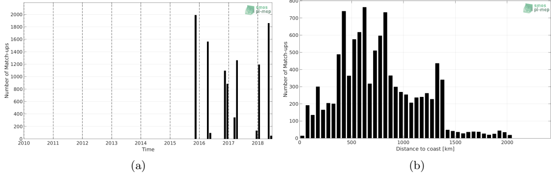
Figure 1: Number of match-ups between TSG-POLARSTERN and SMAP-L3-RSS-V3-8DAY-RUNNING-40KM SSS as a function of time (a) and as function of the distance to coast (b) over the Tropical Atlantic Ocean Pi-MEP region and for the full satellite product period.
