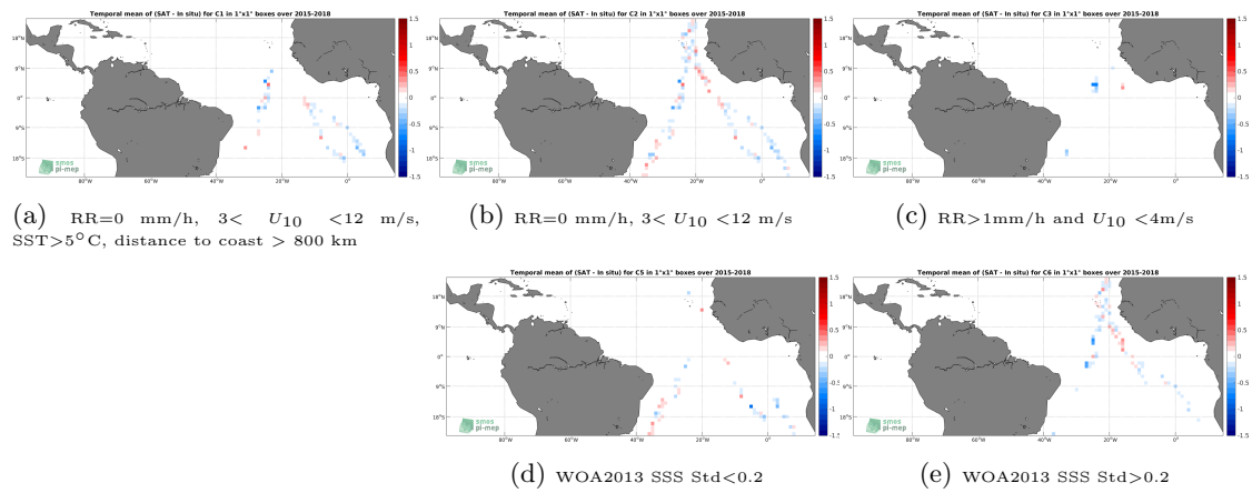
Figure 12: Temporal mean gridded over spatial boxes of size 1^\circ \times 1^\circ of \Delta SSS (SMAP-L3-RSS-V3-8DAY-RUNNING-40KM - TSG-POLARSTERN) for 5 different subdatasets corresponding to:RR=0 mm/h, 3 < U_{10} < 12 m/s, SST >5^\circ C, distance to coast > 800 km (a), RR=0 mm/h, 3 < U_{10} < 12 m/s (b), RR >1 mm/h and U_{10} < 4 m/s (c), WOA2013 SSS Std <0.2 (d), WOA2013 SSS Std >0.2 (e).
