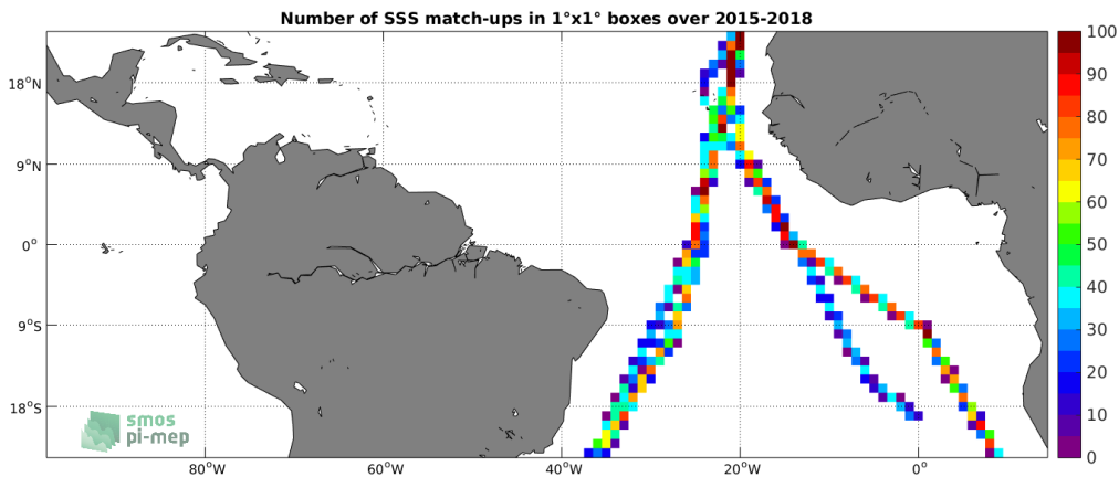
Figure 4: Number of SSS match-ups between TSG-POLARSTERN SSS and the SMAP-L3-RSS-V3-8DAY-RUNNING-40KM SSS product for the Tropical Atlantic Ocean Pi-MEP region over 1^\circ \times 1^\circ boxes and for the full satellite product period.
