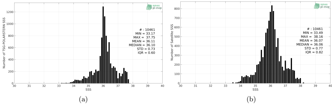
Figure 2: Histograms of SSS from TSG-POLARSTERN (a) and SMAP-L3-RSS-V3-8DAY-RUNNING-40KM (b) considering all match-up pairs per bins of 0.1 over the Tropical Atlantic Ocean Pi-MEP region and for the full satellite product period.
