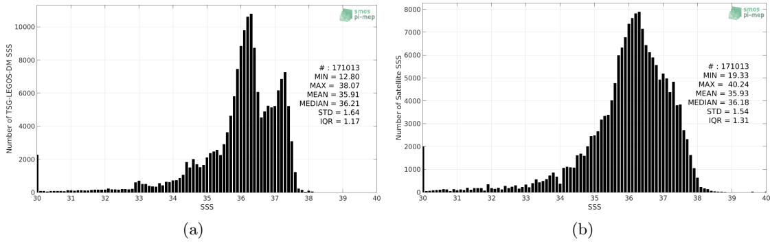
Figure 2: Histograms of SSS from TSG-LEGOS-DM (a) and SMAP-L3-RSS-V3-8DAY-RUNNING-40KM (b) considering all match-up pairs per bins of 0.1 over the Tropical Atlantic Ocean Pi-MEP region and for the full satellite product period.
