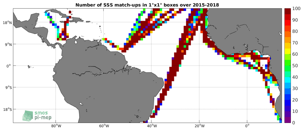
Figure 4: Number of SSS match-ups between TSG-LEGOS-DM SSS and the SMAP-L3-RSS-V3-8DAY-RUNNING-40KM SSS product for the Tropical Atlantic Ocean Pi-MEP region over 1^\circ \times 1^\circ boxes and for the full satellite product period.
