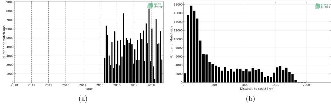
Figure 1: Number of match-ups between TSG-LEGOS-DM and SMAP-L3-RSS-V3-8DAY-RUNNING-40KM SSS as a function of time (a) and as function of the distance to coast (b) over the Tropical Atlantic Ocean Pi-MEP region and for the full satellite product period.
