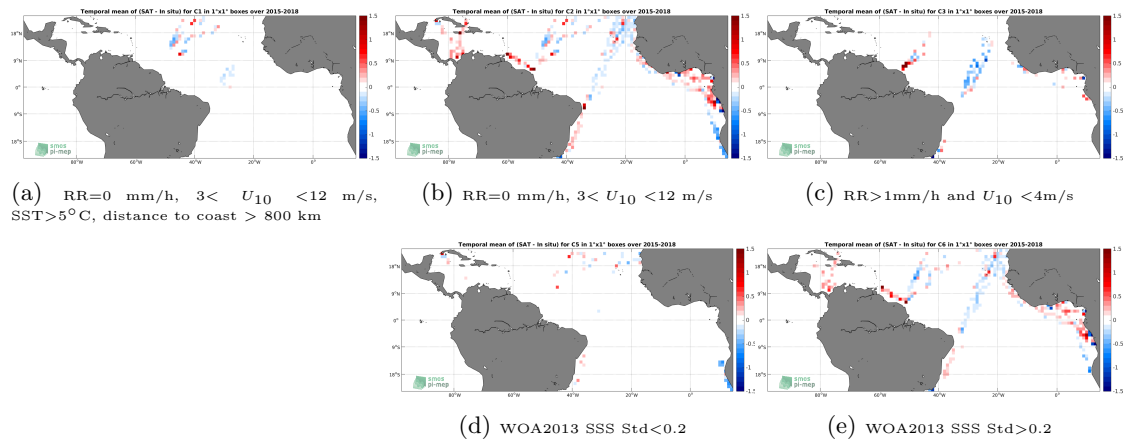
Figure 12: Temporal mean gridded over spatial boxes of size 1^\circ \times 1^\circ of \Delta SSS (SMAP-L3-RSS-V3-8DAY-RUNNING-40KM - TSG-LEGOS-DM) for 5 different subdatasets corresponding to:RR=0 mm/h, 3 < U_{10} < 12 m/s, SST >5^\circ C, distance to coast > 800 km (a), RR=0 mm/h, 3 < U_{10} < 12 m/s (b), RR >1 mm/h and U_{10} < 4 m/s (c), WOA2013 SSS Std <0.2 (d), WOA2013 SSS Std >0.2 (e).
