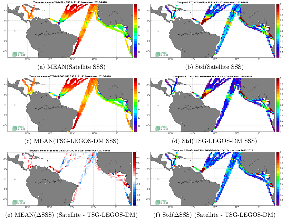
Figure 6: Temporal mean (left) and Std (right) of SSS from SMAP-L3-RSS-V3-8DAY-RUNNING-40KM (top), TSG-LEGOS-DM (middle), and of \Delta SSS (Satellite - TSG-LEGOS-DM). Only match-up pairs are used to generate these maps.
