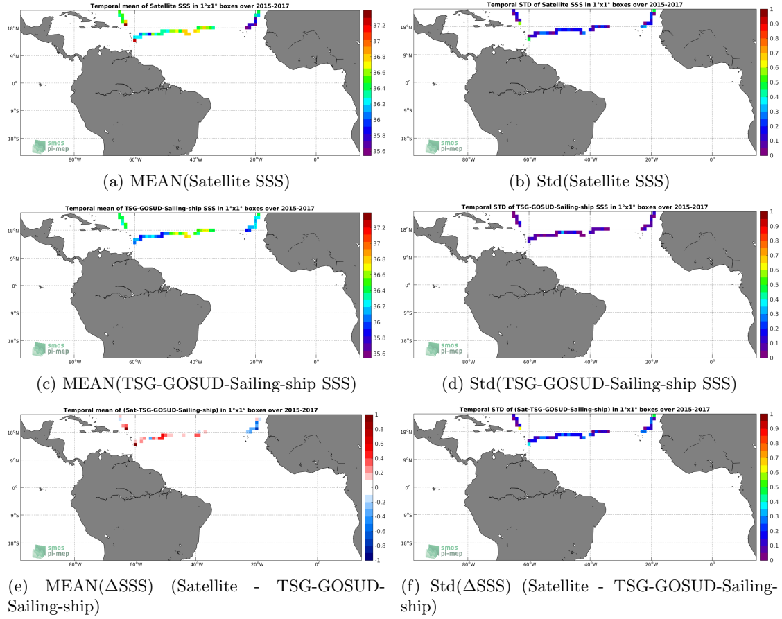
Figure 6: Temporal mean (left) and Std (right) of SSS from SMAP-L3-RSS-V3-8DAY-RUNNING-40KM (top), TSG-GOSUD-Sailing-ship (middle), and of \Delta SSS (Satellite - TSG-GOSUD-Sailing-ship). Only match-up pairs are used to generate these maps.
