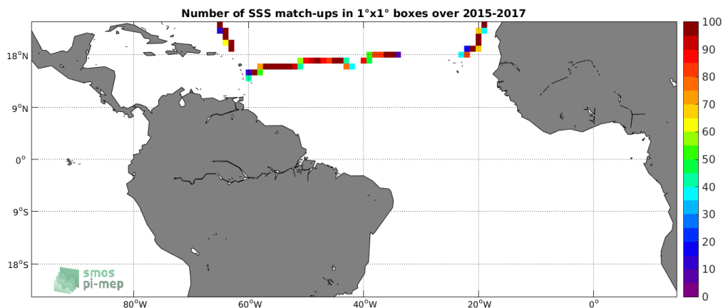
Figure 4: Number of SSS match-ups between TSG-GOSUD-Sailing-ship SSS and the SMAP-L3-RSS-V3-8DAY-RUNNING-40KM SSS product for the Tropical Atlantic Ocean Pi-MEP region over 1^\circ \times 1^\circ boxes and for the full satellite product period.
