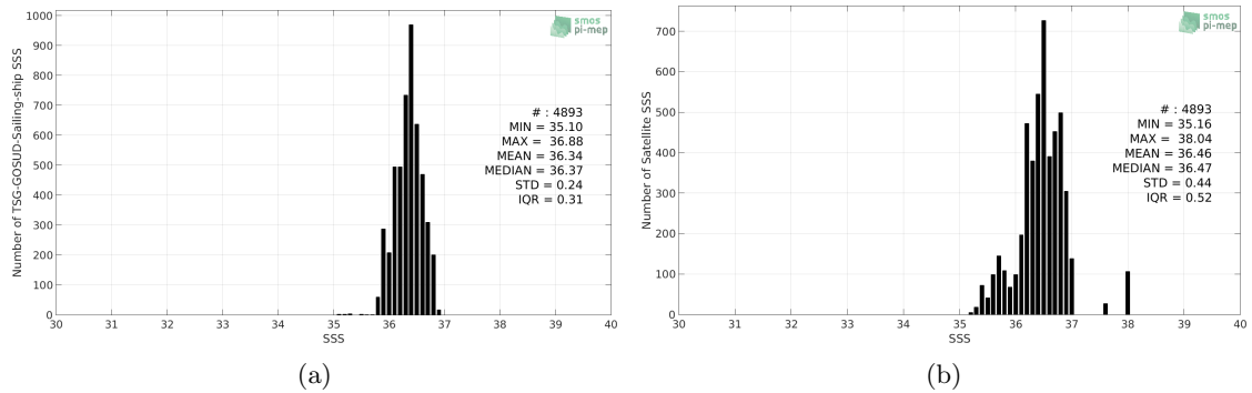
Figure 2: Histograms of SSS from TSG-GOSUD-Sailing-ship (a) and SMAP-L3-RSS-V3-8DAY-RUNNING-40KM (b) considering all match-up pairs per bins of 0.1 over the Tropical Atlantic Ocean Pi-MEP region and for the full satellite product period.
