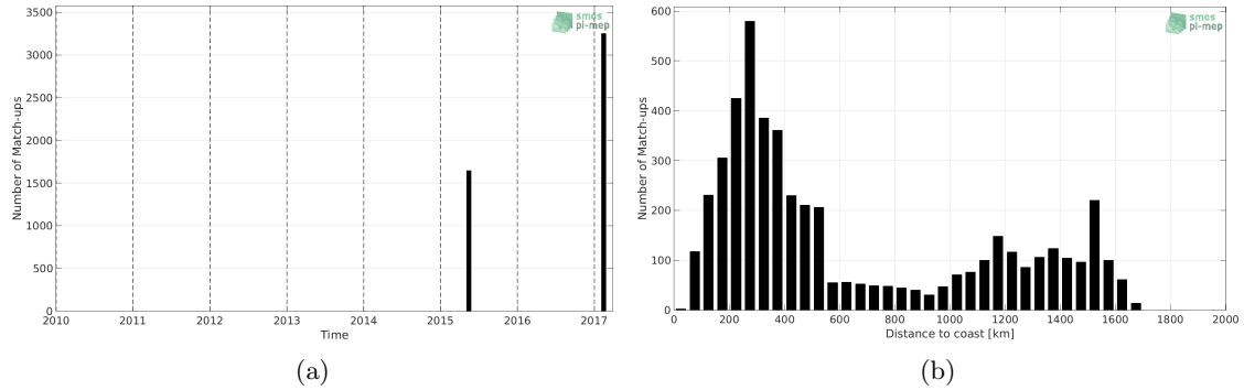
Figure 1: Number of match-ups between TSG-GOSUD-Sailing-ship and SMAP-L3-RSS-V3-8DAY-RUNNING-40KM SSS as a function of time (a) and as function of the distance to coast (b) over the Tropical Atlantic Ocean Pi-MEP region and for the full satellite product period.
