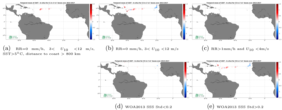
Figure 12: Temporal mean gridded over spatial boxes of size 1^\circ \times 1^\circ of \Delta SSS (SMAP-L3-RSS-V3-8DAY-RUNNING-40KM - TSG-GOSUD-Sailing-ship) for 5 different subdatasets corresponding to:RR=0 mm/h, 3 < U_{10} < 12 m/s, SST >5^\circ C, distance to coast > 800 km (a), RR=0 mm/h, 3 < U_{10} < 12 m/s (b), RR >1 mm/h and U_{10} < 4 m/s (c), WOA2013 SSS Std <0.2 (d), WOA2013 SSS Std >0.2 (e).
