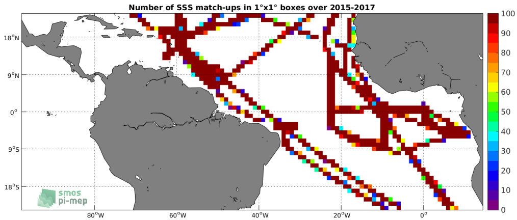
Figure 4: Number of SSS match-ups between TSG-GOSUD-Research-vessel SSS and the SMAP-L3-RSS-V3-8DAY-RUNNING-40KM SSS product for the Tropical Atlantic Ocean Pi-MEP region over 1^\circ \times 1^\circ boxes and for the full satellite product period.
