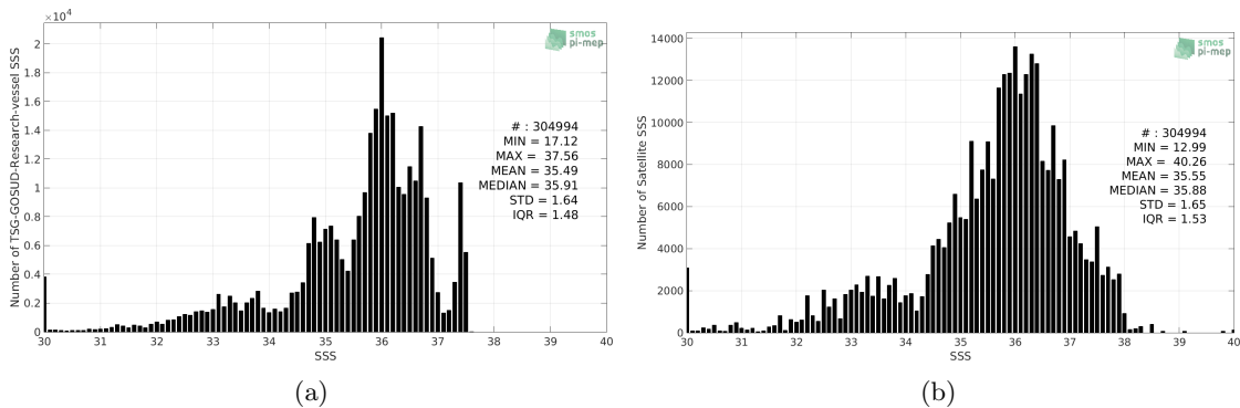
Figure 2: Histograms of SSS from TSG-GOSUD-Research-vessel (a) and SMAP-L3-RSS-V3-8DAY-RUNNING-40KM (b) considering all match-up pairs per bins of 0.1 over the Tropical Atlantic Ocean Pi-MEP region and for the full satellite product period.
