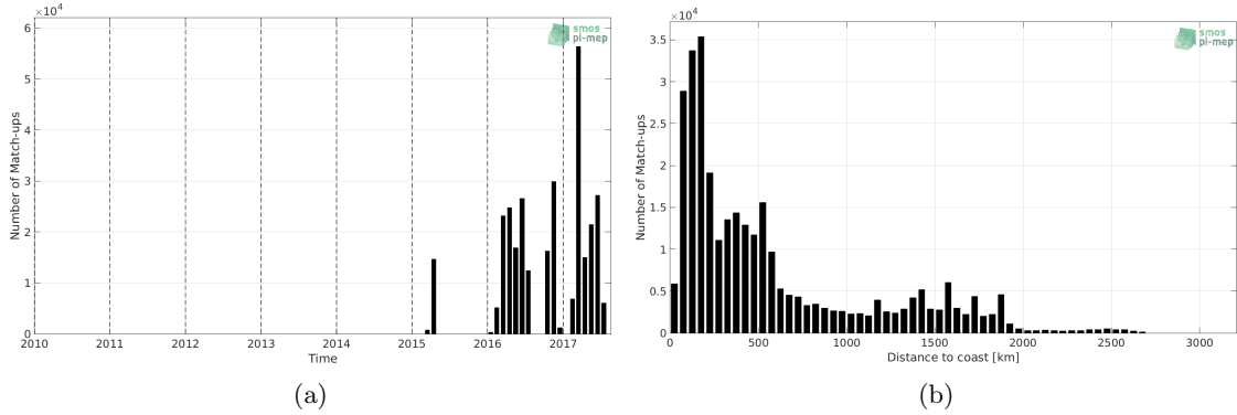
Figure 1: Number of match-ups between TSG-GOSUD-Research-vessel and SMAP-L3-RSS-V3-8DAY-RUNNING-40KM SSS as a function of time (a) and as function of the distance to coast (b) over the Tropical Atlantic Ocean Pi-MEP region and for the full satellite product period.
