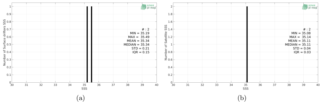
Figure 2: Histograms of SSS from Surface drifters (a) and SMAP-L3-RSS-V3-8DAY-RUNNING-40KM (b) considering all match-up pairs per bins of 0.1 over the Tropical Atlantic Ocean Pi-MEP region and for the full satellite product period.
