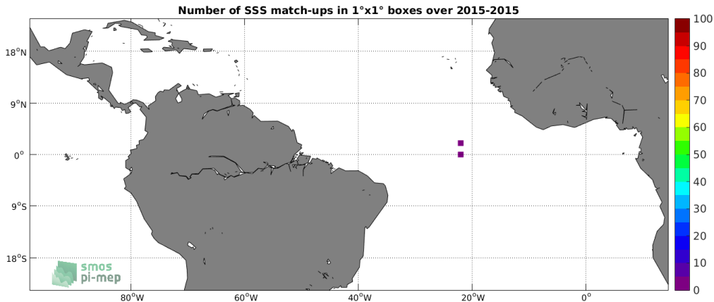
Figure 3: Number of SSS match-ups between Surface drifters SSS and the SMAP-L3-RSS-V3-8DAY-RUNNING-40KM SSS product for the Tropical Atlantic Ocean Pi-MEP region over 1^\circ \times 1^\circ boxes and for the full satellite product period.
