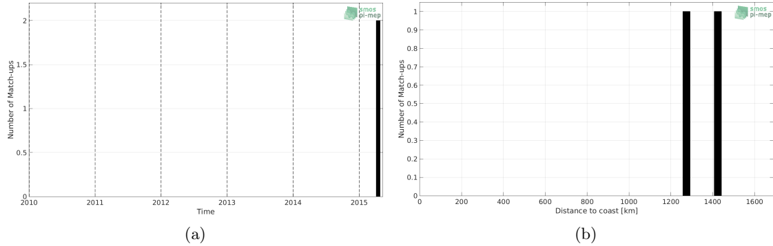
Figure 1: Number of match-ups between Surface drifters and SMAP-L3-RSS-V3-8DAY-RUNNING-40KM SSS as a function of time (a) and as function of the distance to coast (b) over the Tropical Atlantic Ocean Pi-MEP region and for the full satellite product period.
