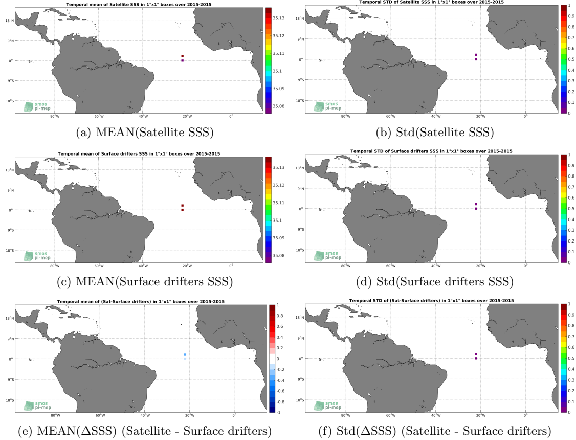
Figure 5: Temporal mean (left) and Std (right) of SSS from SMAP-L3-RSS-V3-8DAY-RUNNING-40KM (top), Surface drifters (middle), and of \Delta SSS (Satellite - Surface drifters). Only match-up pairs are used to generate these maps.
