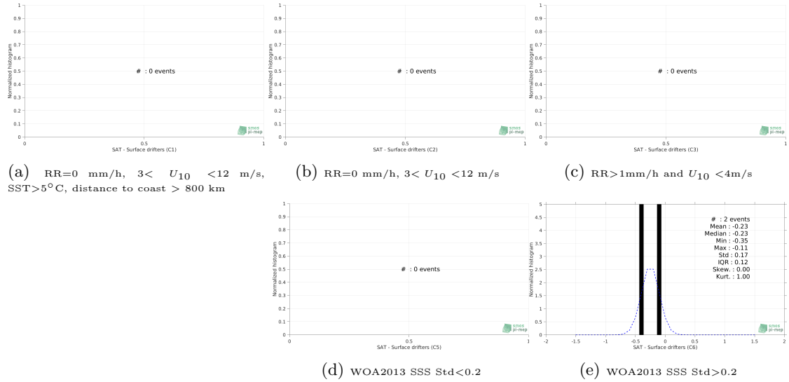
Figure 12: Normalized histogram of \Delta\text{SSS} (SMAP-L3-RSS-V3-8DAY-RUNNING-40KM - Surface drifters) for 5 different subdatasets corresponding to: RR=0 mm/h, 3 < U_{10} < 12 m/s, SST > 5^\circ\text{C} , distance to coast > 800 km (a), RR=0 mm/h, 3 < U_{10} < 12 m/s (b), RR > 1\text{mm/h} and U_{10} < 4\text{m/s} (c), WOA2013 SSS Std < 0.2 (d), WOA2013 SSS Std > 0.2 (e).
