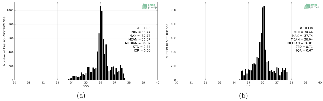
Figure 2: Histograms of SSS from TSG-POLARSTERN (a) and SMAP-L3-RSS-V3-MONTHLY-70KM (b) considering all match-up pairs per bins of 0.1 over the Tropical Atlantic Ocean Pi-MEP region and for the full satellite product period.
