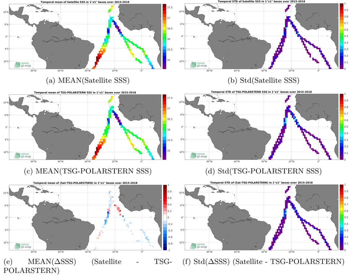
Figure 6: Temporal mean (left) and Std (right) of SSS from SMAP-L3-RSS-V3-MONTHLY-70KM (top), TSG-POLARSTERN (middle), and of \Delta SSS (Satellite - TSG-POLARSTERN). Only match-up pairs are used to generate these maps.
