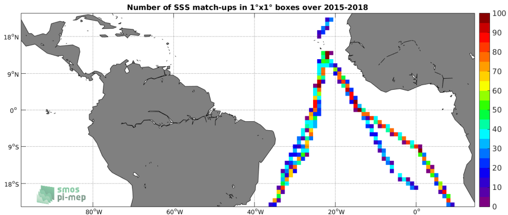
Figure 4: Number of SSS match-ups between TSG-POLARSTERN SSS and the SMAP-L3-RSS-V3-MONTHLY-70KM SSS product for the Tropical Atlantic Ocean Pi-MEP region over 1^\circ \times 1^\circ boxes and for the full satellite product period.
