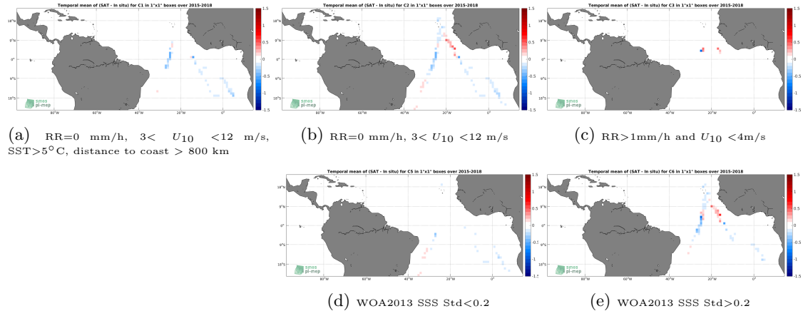
Figure 12: Temporal mean gridded over spatial boxes of size 1^\circ \times 1^\circ of \Delta SSS (SMAP-L3-RSS-V3-MONTHLY-70KM - TSG-POLARSTERN) for 5 different subdatasets corresponding to: RR=0 mm/h, 3 < U_{10} < 12 m/s, SST > 5^\circ C , distance to coast > 800 km (a), RR=0 mm/h, 3 < U_{10} < 12 m/s (b), RR > 1 mm/h and U_{10} < 4 m/s (c), WOA2013 SSS Std < 0.2 (d), WOA2013 SSS Std > 0.2 (e).
