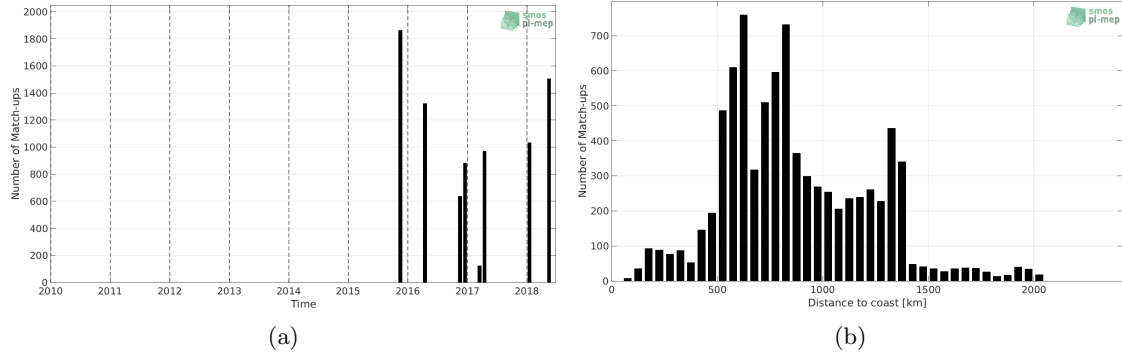
Figure 1: Number of match-ups between TSG-POLARSTERN and SMAP-L3-RSS-V3-MONTHLY-70KM SSS as a function of time (a) and as function of the distance to coast (b) over the Tropical Atlantic Ocean Pi-MEP region and for the full satellite product period.
