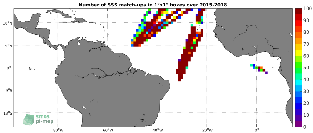
Figure 4: Number of SSS match-ups between TSG-LEGOS-DM SSS and the SMAP-L3-RSS-V3-MONTHLY-70KM SSS product for the Tropical Atlantic Ocean Pi-MEP region over 1^\circ \times 1^\circ boxes and for the full satellite product period.
