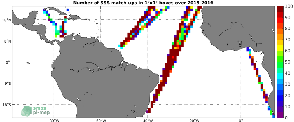
Figure 4: Number of SSS match-ups between TSG-LEGOS-DM SSS and the SMAP-L3-RSS-V3-MONTHLY-70KM SSS product for the Tropical Atlantic Ocean Pi-MEP region over 1^\circ \times 1^\circ boxes and for the full satellite product period.
