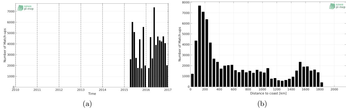
Figure 1: Number of match-ups between TSG-LEGOS-DM and SMAP-L3-RSS-V3-MONTHLY-70KM SSS as a function of time (a) and as function of the distance to coast (b) over the Tropical Atlantic Ocean Pi-MEP region and for the full satellite product period.
