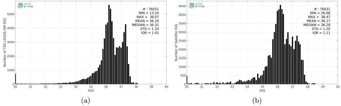
Figure 2: Histograms of SSS from TSG-LEGOS-DM (a) and SMAP-L3-RSS-V3-MONTHLY-70KM (b) considering all match-up pairs per bins of 0.1 over the Tropical Atlantic Ocean Pi-MEP region and for the full satellite product period.
