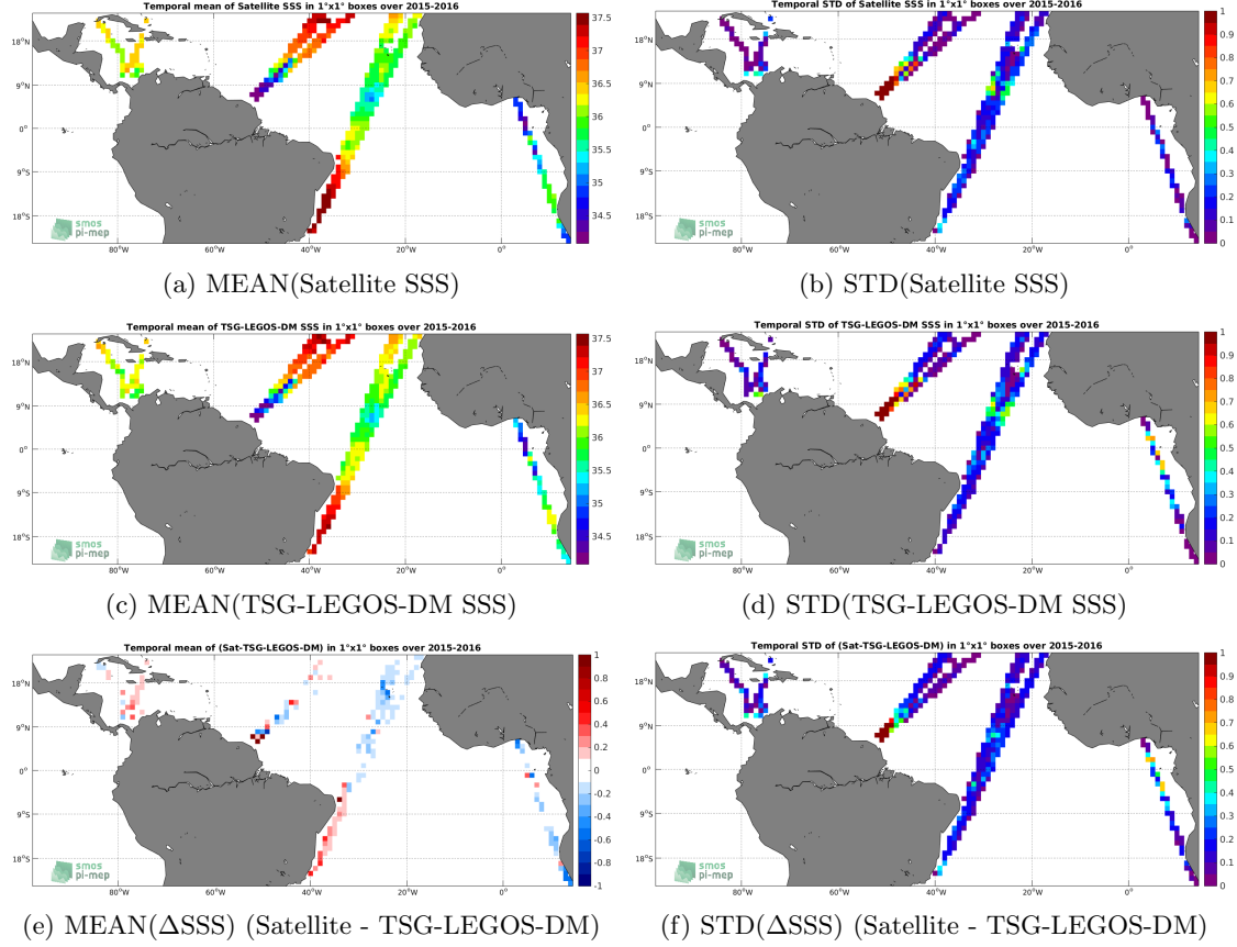
Figure 6: Temporal mean (left) and STD (right) of SSS from SMAP-L3-RSS-V3-MONTHLY-70KM (top), TSG-LEGOS-DM (middle), and of \Delta SSS (Satellite - TSG-LEGOS-DM). Only match-up pairs are used to generate these maps.
