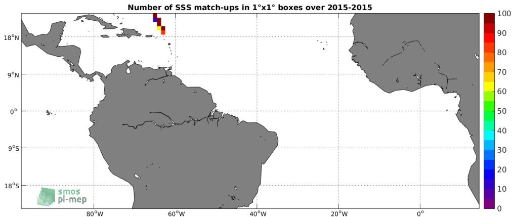
Figure 4: Number of SSS match-ups between TSG-GOSUD-Sailing-ship SSS and the SMAP-L3-RSS-V3-MONTHLY-70KM SSS product for the Tropical Atlantic Ocean Pi-MEP region over 1^\circ \times 1^\circ boxes and for the full satellite product period.
