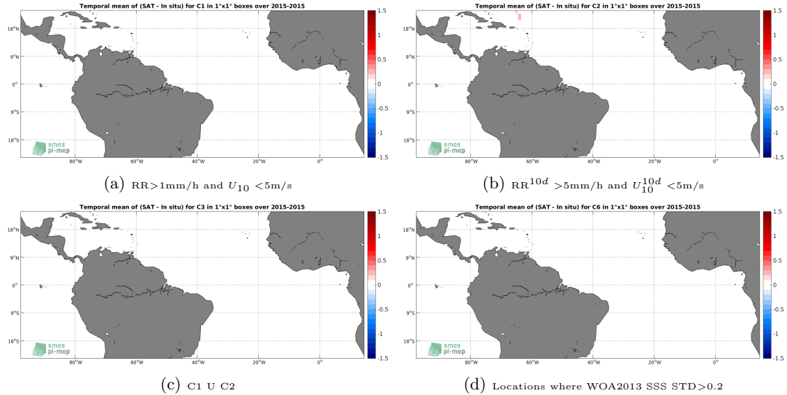
Figure 12: Temporal mean gridded over spatial boxes of size 1^\circ \times 1^\circ of \Delta SSS (SMAP-L3-RSS-V3-MONTHLY-70KM - TSG-GOSUD-Sailing-ship) for 4 different subdatasets corresponding to: RR > 1mm/h and U_{10} < 5\text{m/s} (a), RR^{10d} > 5\text{mm/h} and U_{10}^{10d} < 5\text{m/s} (b), C1 U C2 (c), Locations where WOA2013 SSS STD > 0.2 (d).
